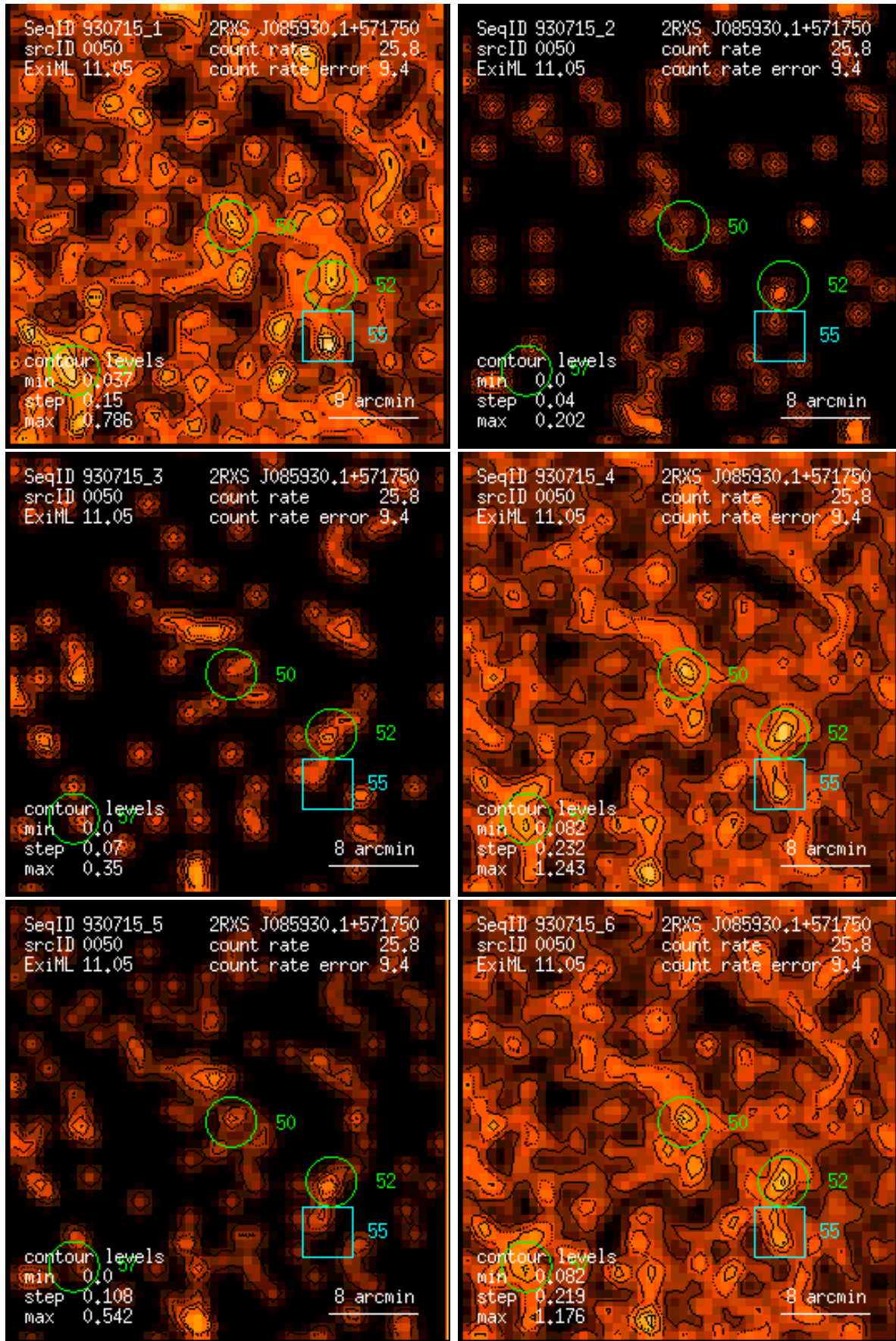
Figure 50: RASS 930715: detection 0050: band rate images, Gaussian filter: (1) PSPC channels 11 – 41, (2) 52 – 90, (3) 91 – 201, (4) 11 – 235, (5) 52 – 201, (6) 11 – 201. Broad band rates in counts/ks. Band rate contour levels in counts/ks/arcmin 2 .
