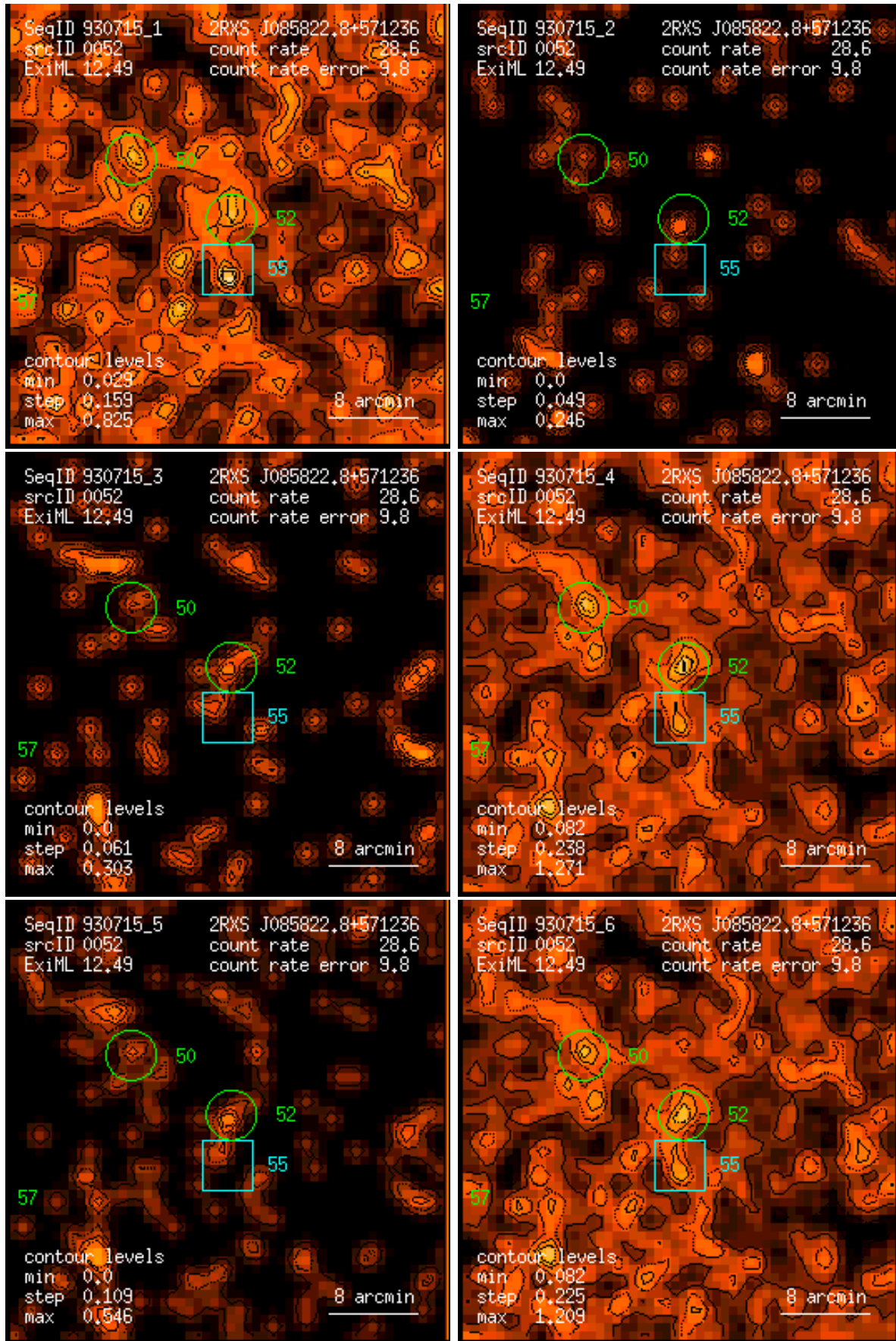
Figure 52: RASS 930715: detection 0052: band rate images, Gaussian filter: (1) PSPC channels 11 – 41, (2) 52 – 90, (3) 91 – 201, (4) 11 – 235, (5) 52 – 201, (6) 11 – 201. Broad band rates in counts/ks. Band rate contour levels in counts/ks/arcmin 2 .
