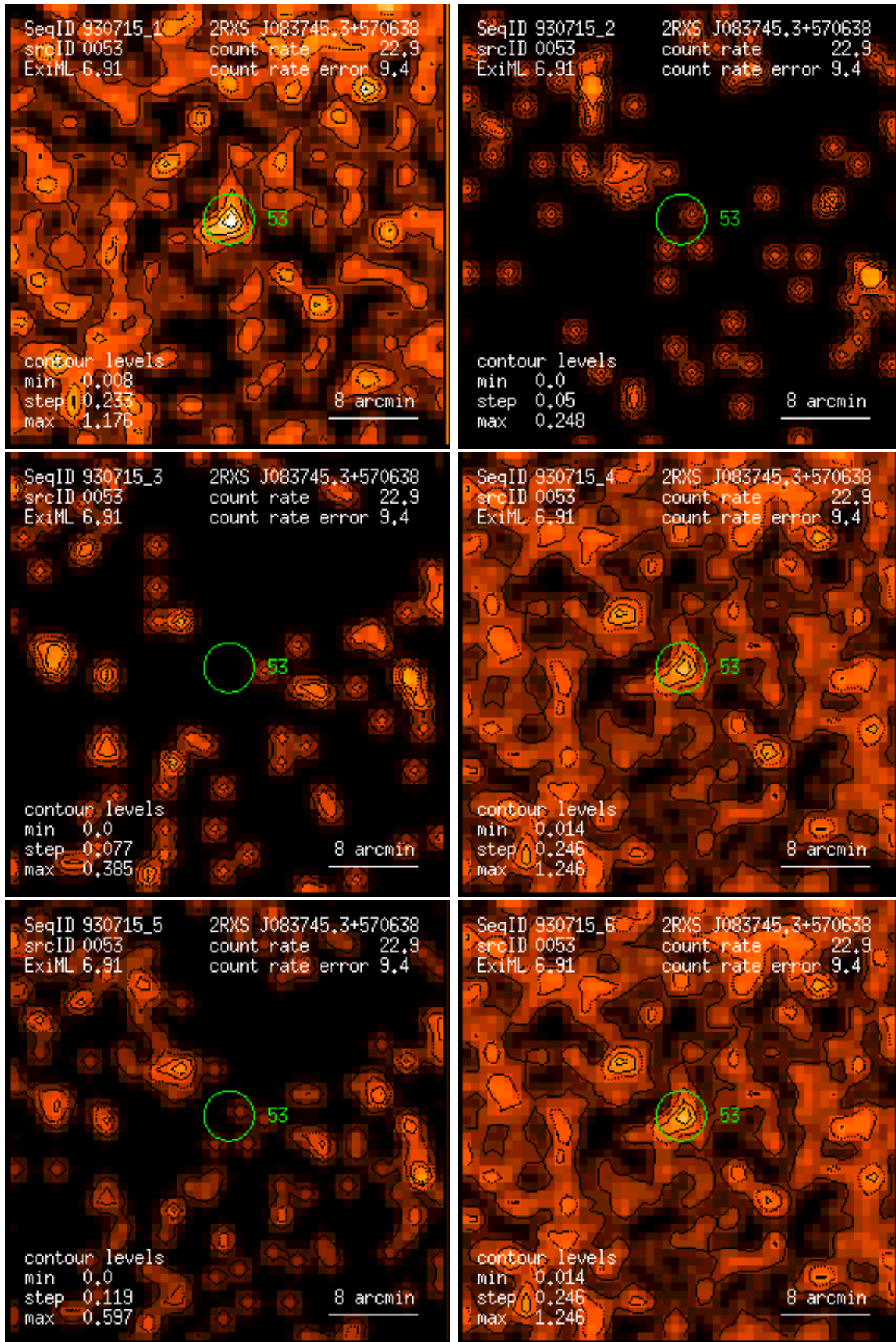
Figure 53: RASS 930715: detection 0053: band rate images, Gaussian filter: (1) PSPC channels 11 – 41, (2) 52 – 90, (3) 91 – 201, (4) 11 – 235, (5) 52 – 201, (6) 11 – 201. Broad band rates in counts/ks. Band rate contour levels in counts/ks/arcmin 2 .
