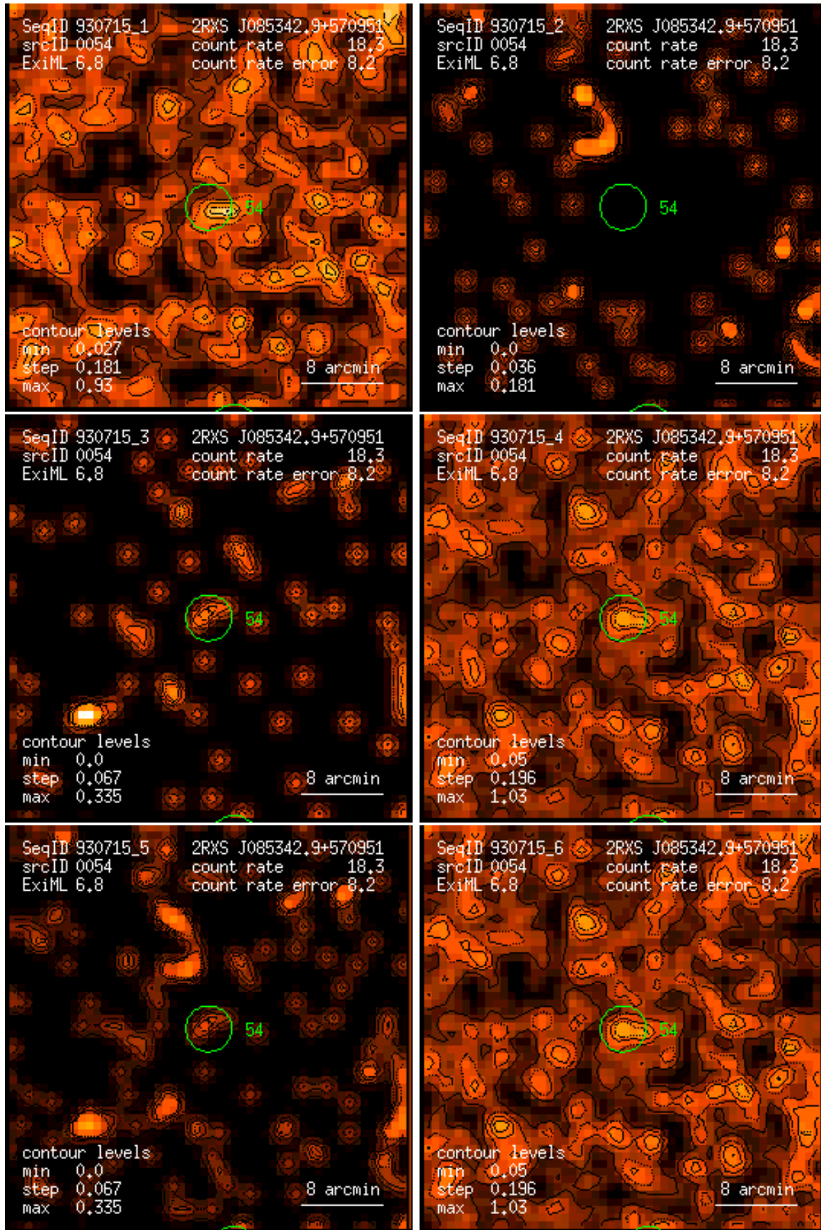
Figure 54: RASS 930715: detection 0054: band rate images, Gaussian filter: (1) PSPC channels 11 – 41, (2) 52 – 90, (3) 91 – 201, (4) 11 – 235, (5) 52 – 201, (6) 11 – 201. Broad band rates in counts/ks. Band rate contour levels in counts/ks/arcmin 2 .
