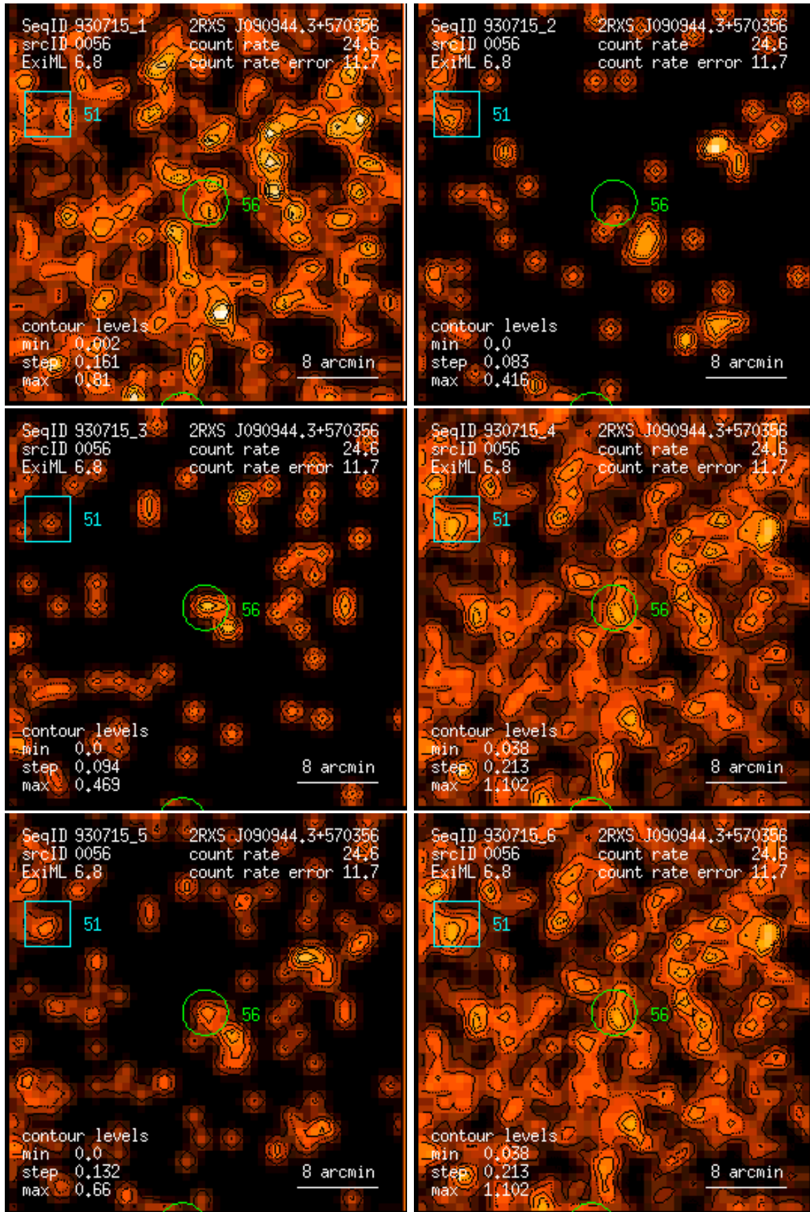
Figure 56: RASS 930715: detection 0056: band rate images, Gaussian filter: (1) PSPC channels 11 – 41, (2) 52 – 90, (3) 91 – 201, (4) 11 – 235, (5) 52 – 201, (6) 11 – 201. Broad band rates in counts/ks. Band rate contour levels in counts/ks/arcmin 2 .
