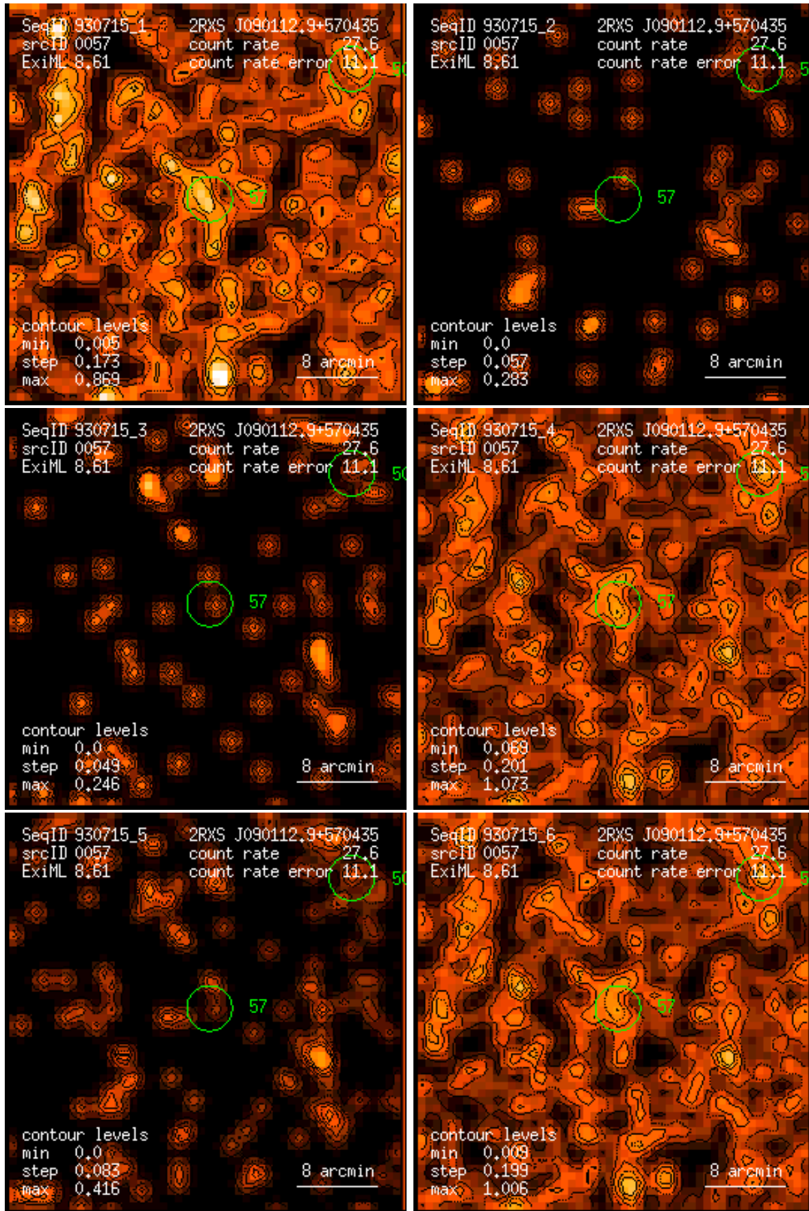
Figure 57: RASS 930715: detection 0057: band rate images, Gaussian filter: (1) PSPC channels 11 – 41, (2) 52 – 90, (3) 91 – 201, (4) 11 – 235, (5) 52 – 201, (6) 11 – 201. Broad band rates in counts/ks. Band rate contour levels in counts/ks/arcmin 2 .
