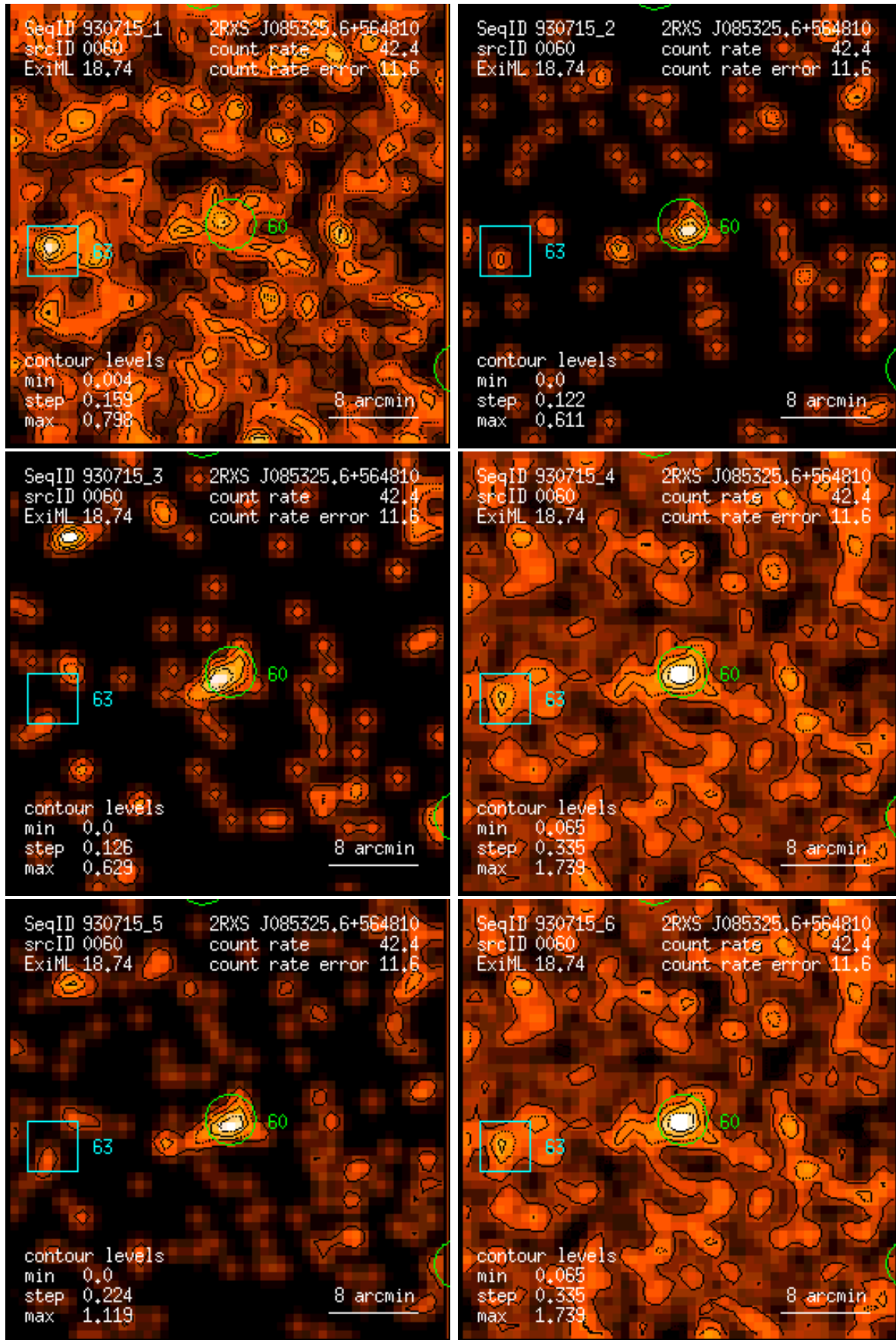
Figure 60: RASS 930715: detection 0060: band rate images, Gaussian filter: (1) PSPC channels 11 – 41, (2) 52 – 90, (3) 91 – 201, (4) 11 – 235, (5) 52 – 201, (6) 11 – 201. Broad band rates in counts/ks. Band rate contour levels in counts/ks/arcmin 2 .
