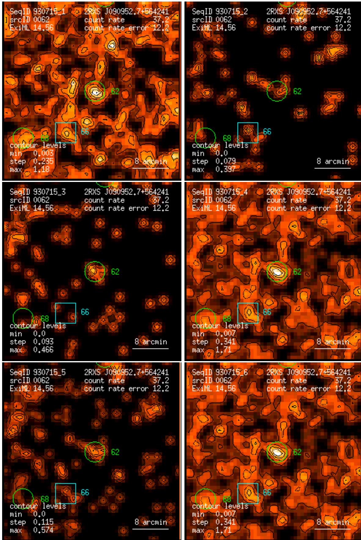
Figure 62: RASS 930715: detection 0062: band rate images, Gaussian filter: (1) PSPC channels 11 – 41, (2) 52 – 90, (3) 91 – 201, (4) 11 – 235, (5) 52 – 201, (6) 11 – 201. Broad band rates in counts/ks. Band rate contour levels in counts/ks/arcmin 2 .
