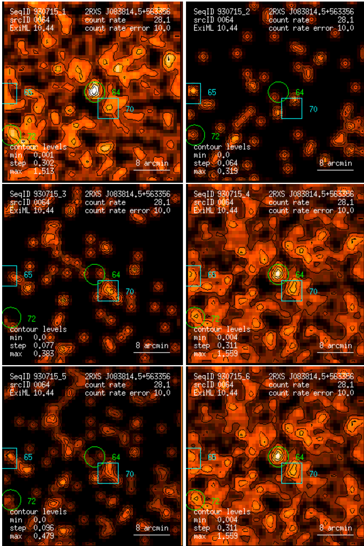
Figure 64: RASS 930715: detection 0064: band rate images, Gaussian filter: (1) PSPC channels 11 – 41, (2) 52 – 90, (3) 91 – 201, (4) 11 – 235, (5) 52 – 201, (6) 11 – 201. Broad band rates in counts/ks. Band rate contour levels in counts/ks/arcmin 2 .
