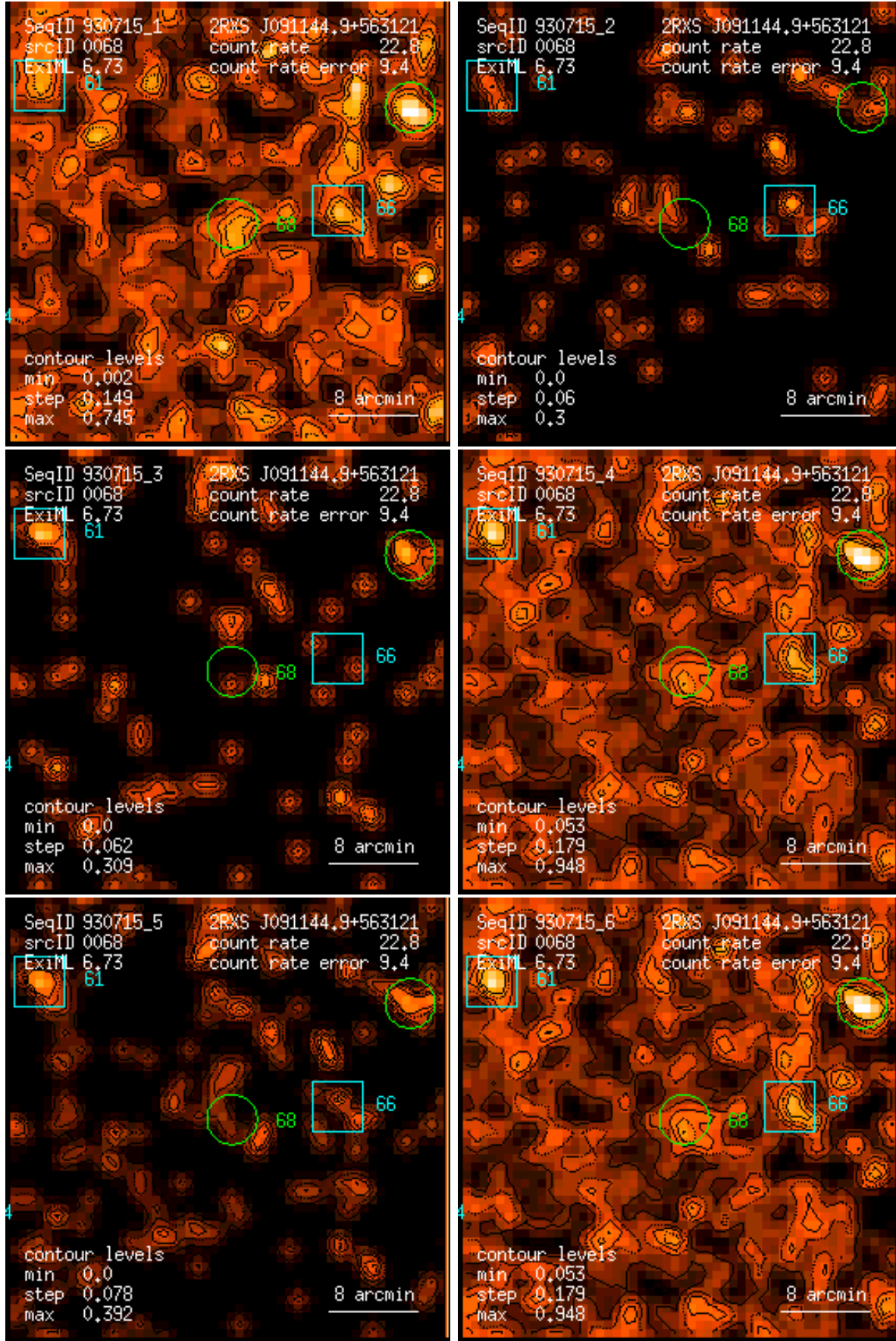
Figure 68: RASS 930715: detection 0068: band rate images, Gaussian filter: (1) PSPC channels 11 – 41, (2) 52 – 90, (3) 91 – 201, (4) 11 – 235, (5) 52 – 201, (6) 11 – 201. Broad band rates in counts/ks. Band rate contour levels in counts/ks/arcmin 2 .
