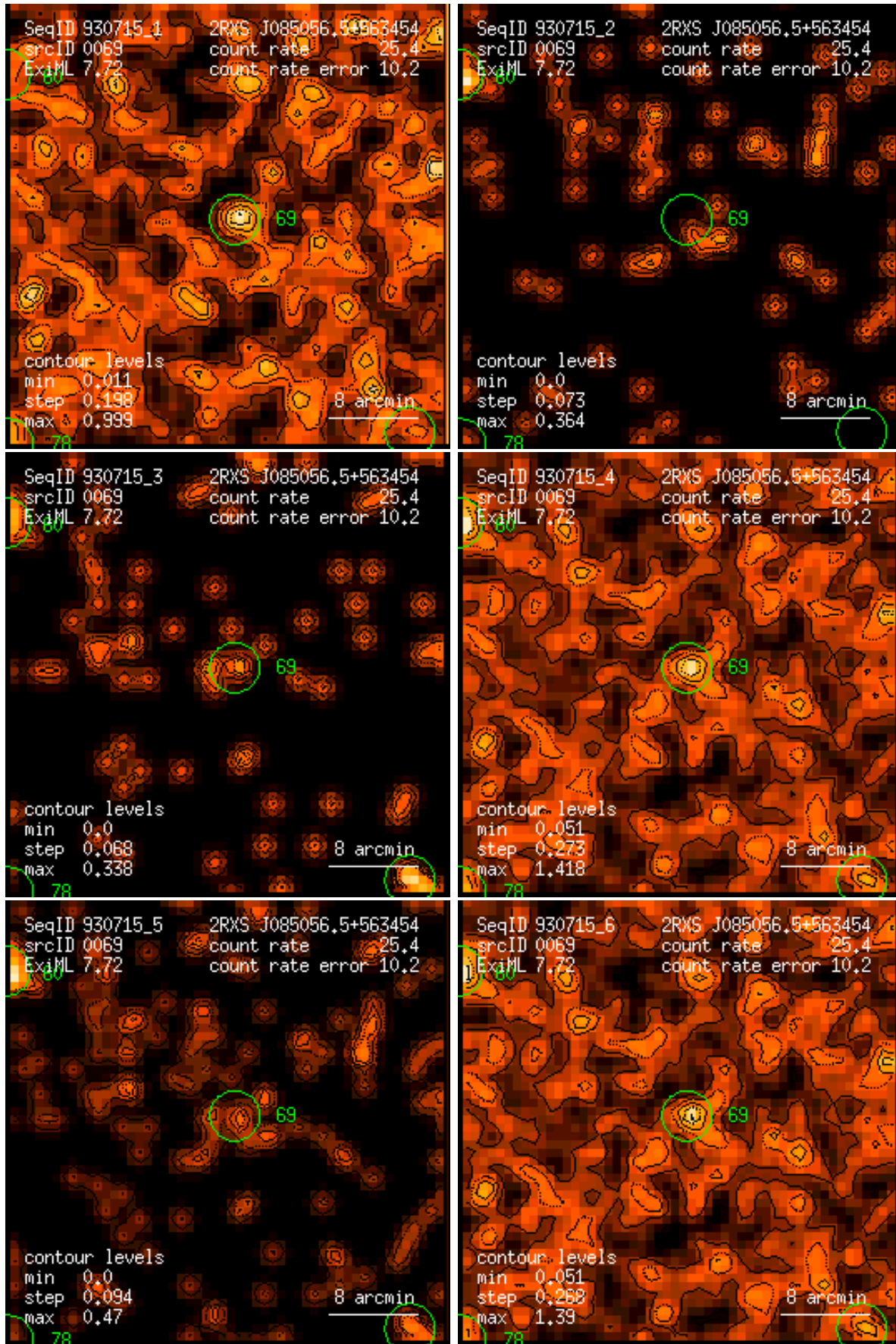
Figure 69: RASS 930715: detection 0069: band rate images, Gaussian filter: (1) PSPC channels 11 – 41, (2) 52 – 90, (3) 91 – 201, (4) 11 – 235, (5) 52 – 201, (6) 11 – 201. Broad band rates in counts/ks. Band rate contour levels in counts/ks/arcmin 2 .
