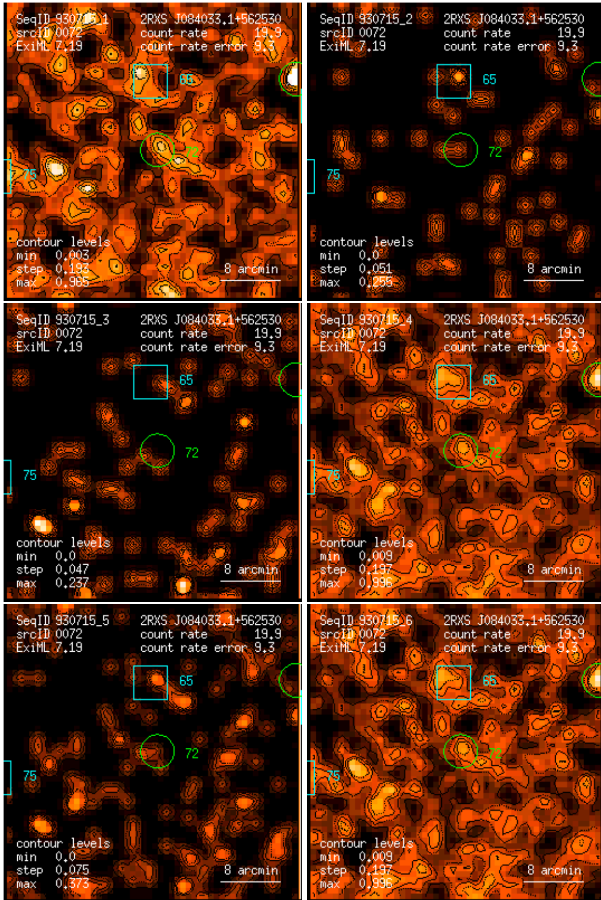
Figure 72: RASS 930715: detection 0072: band rate images, Gaussian filter: (1) PSPC channels 11 – 41, (2) 52 – 90, (3) 91 – 201, (4) 11 – 235, (5) 52 – 201, (6) 11 – 201. Broad band rates in counts/ks. Band rate contour levels in counts/ks/arcmin 2 .
