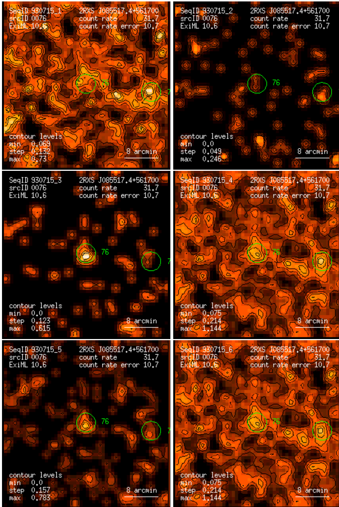
Figure 76: RASS 930715: detection 0076: band rate images, Gaussian filter: (1) PSPC channels 11 – 41, (2) 52 – 90, (3) 91 – 201, (4) 11 – 235, (5) 52 – 201, (6) 11 – 201. Broad band rates in counts/ks. Band rate contour levels in counts/ks/arcmin 2 .
