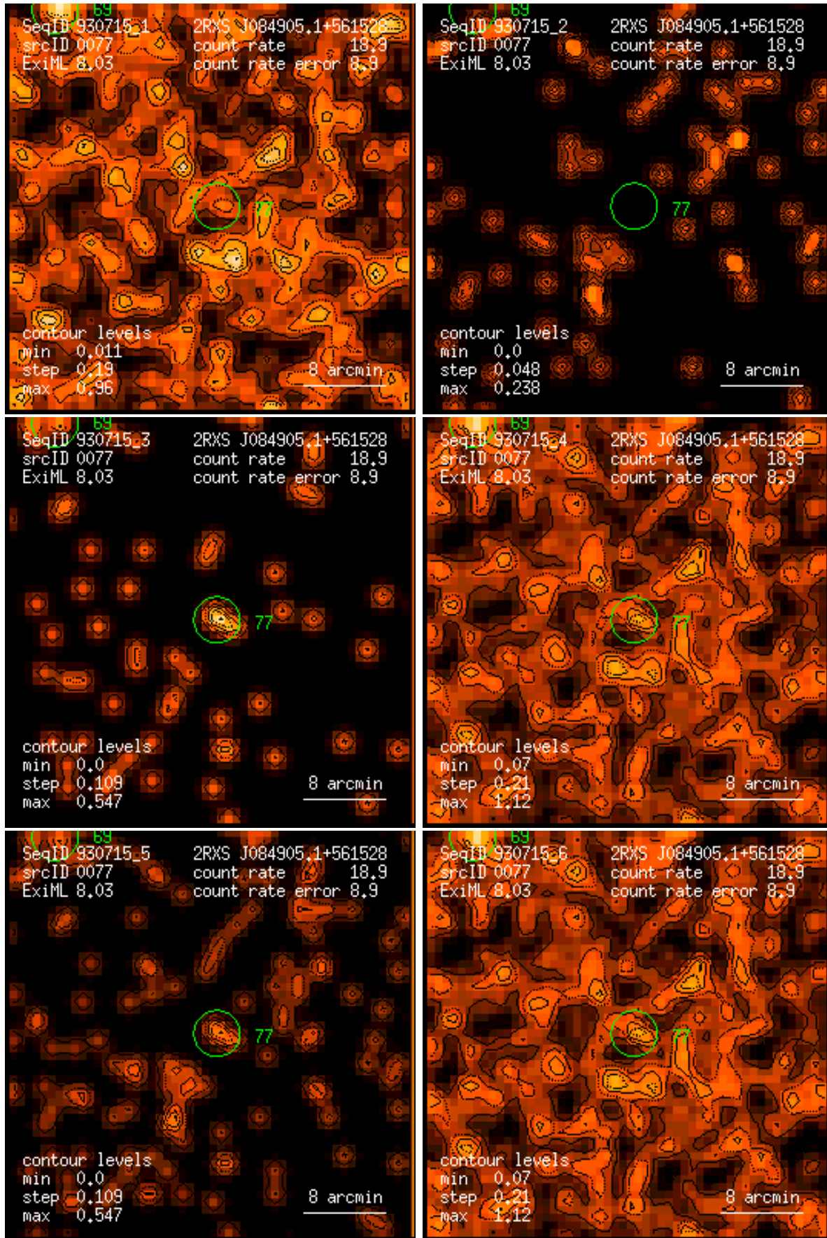
Figure 77: RASS 930715: detection 0077: band rate images, Gaussian filter: (1) PSPC channels 11 – 41, (2) 52 – 90, (3) 91 – 201, (4) 11 – 235, (5) 52 – 201, (6) 11 – 201. Broad band rates in counts/ks. Band rate contour levels in counts/ks/arcmin 2 .
