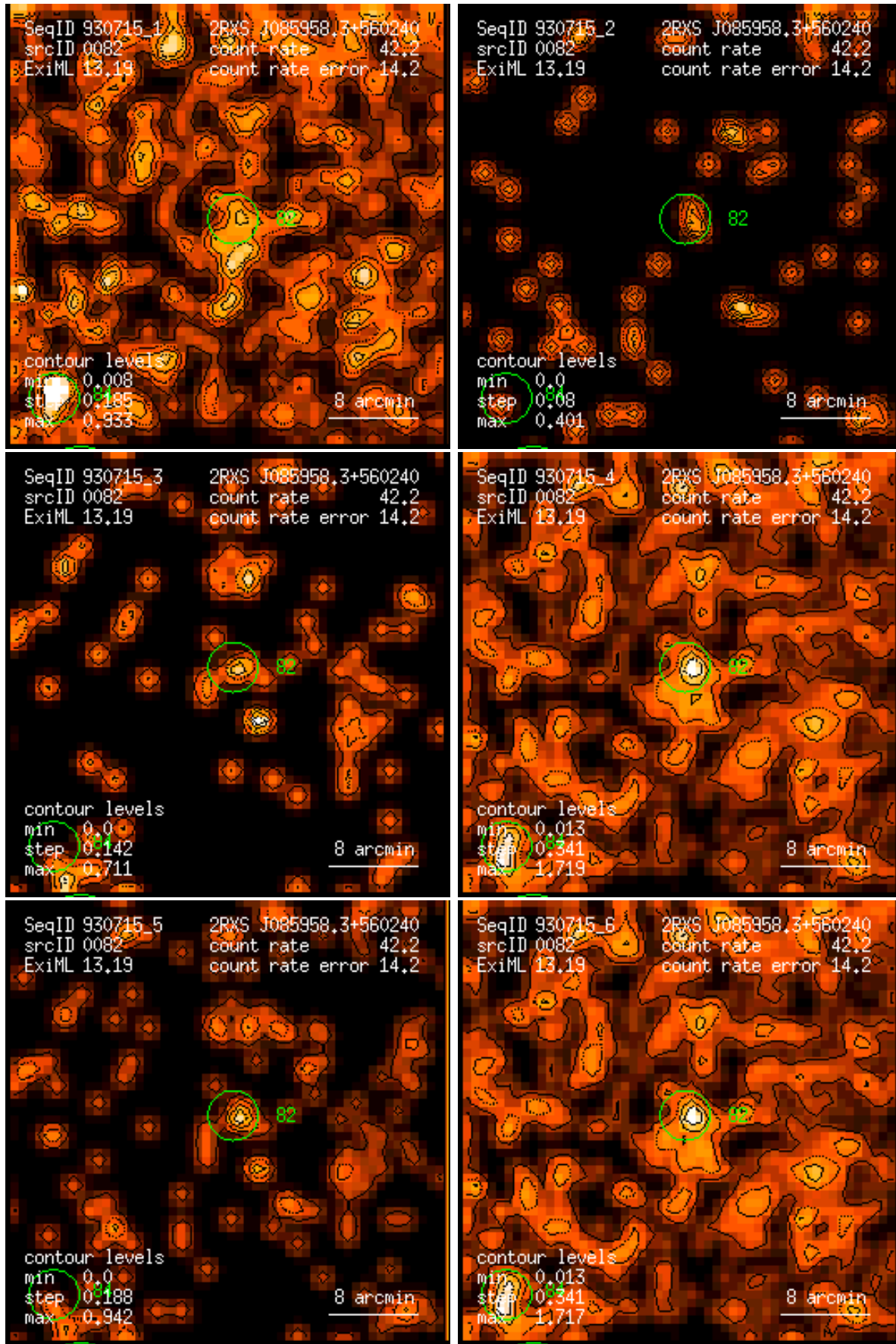
Figure 82: RASS 930715: detection 0082: band rate images, Gaussian filter: (1) PSPC channels 11 – 41, (2) 52 – 90, (3) 91 – 201, (4) 11 – 235, (5) 52 – 201, (6) 11 – 201. Broad band rates in counts/ks. Band rate contour levels in counts/ks/arcmin 2 .
