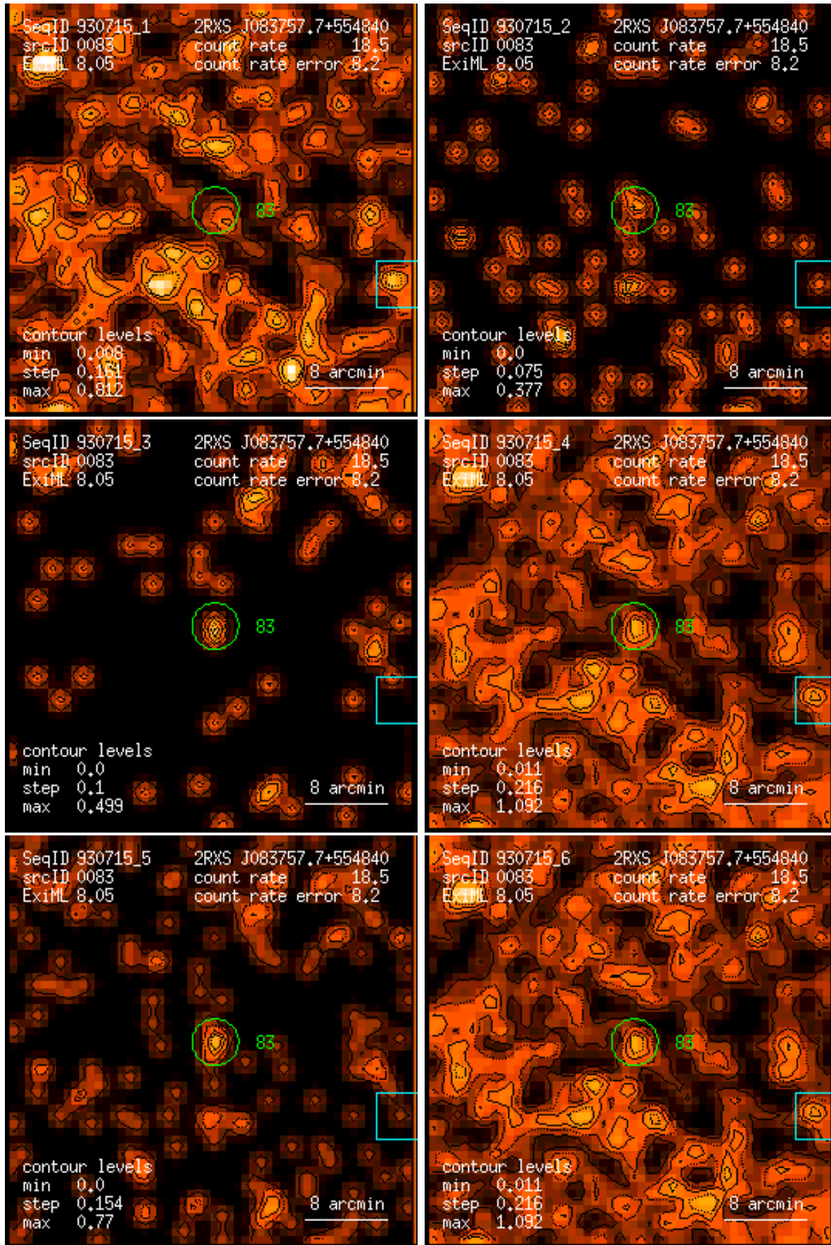
Figure 83: RASS 930715: detection 0083: band rate images, Gaussian filter: (1) PSPC channels 11 – 41, (2) 52 – 90, (3) 91 – 201, (4) 11 – 235, (5) 52 – 201, (6) 11 – 201. Broad band rates in counts/ks. Band rate contour levels in counts/ks/arcmin 2 .
