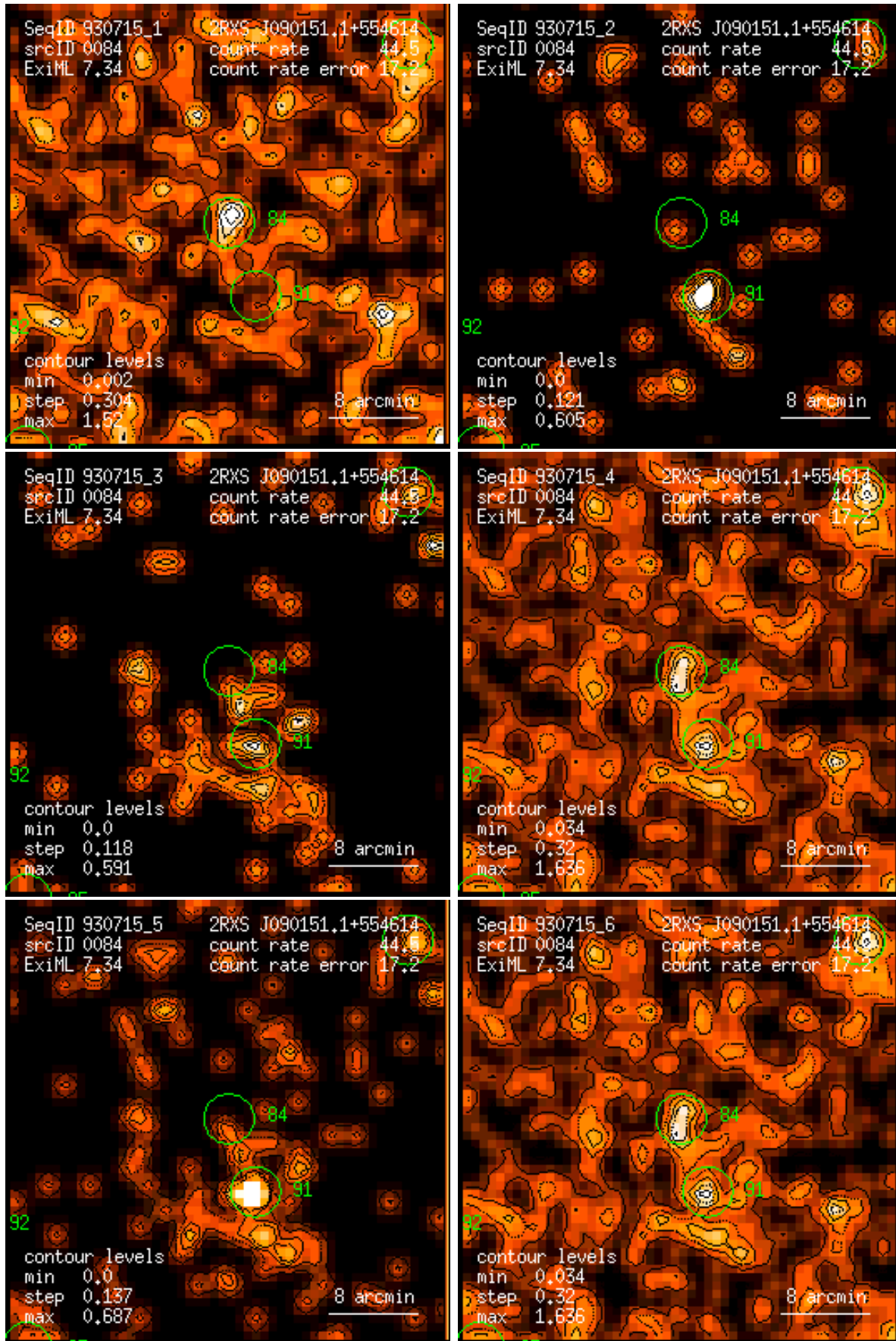
Figure 84: RASS 930715: detection 0084: band rate images, Gaussian filter: (1) PSPC channels 11 – 41, (2) 52 – 90, (3) 91 – 201, (4) 11 – 235, (5) 52 – 201, (6) 11 – 201. Broad band rates in counts/ks. Band rate contour levels in counts/ks/arcmin 2 .
