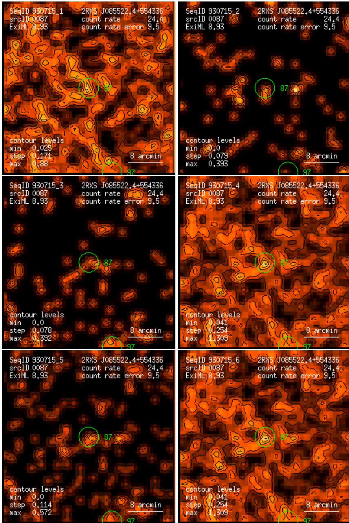
Figure 87: RASS 930715: detection 0087: band rate images, Gaussian filter: (1) PSPC channels 11 – 41, (2) 52 – 90, (3) 91 – 201, (4) 11 – 235, (5) 52 – 201, (6) 11 – 201. Broad band rates in counts/ks. Band rate contour levels in counts/ks/arcmin 2 .
