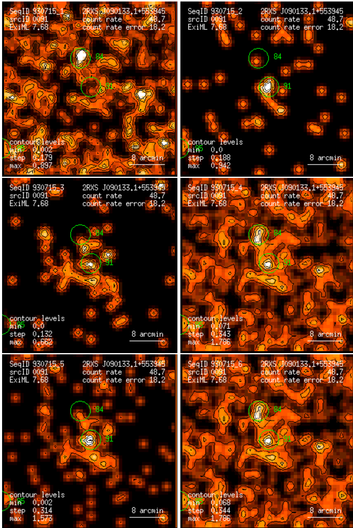
Figure 91: RASS 930715: detection 0091: band rate images, Gaussian filter: (1) PSPC channels 11 – 41, (2) 52 – 90, (3) 91 – 201, (4) 11 – 235, (5) 52 – 201, (6) 11 – 201. Broad band rates in counts/ks. Band rate contour levels in counts/ks/arcmin 2 .
