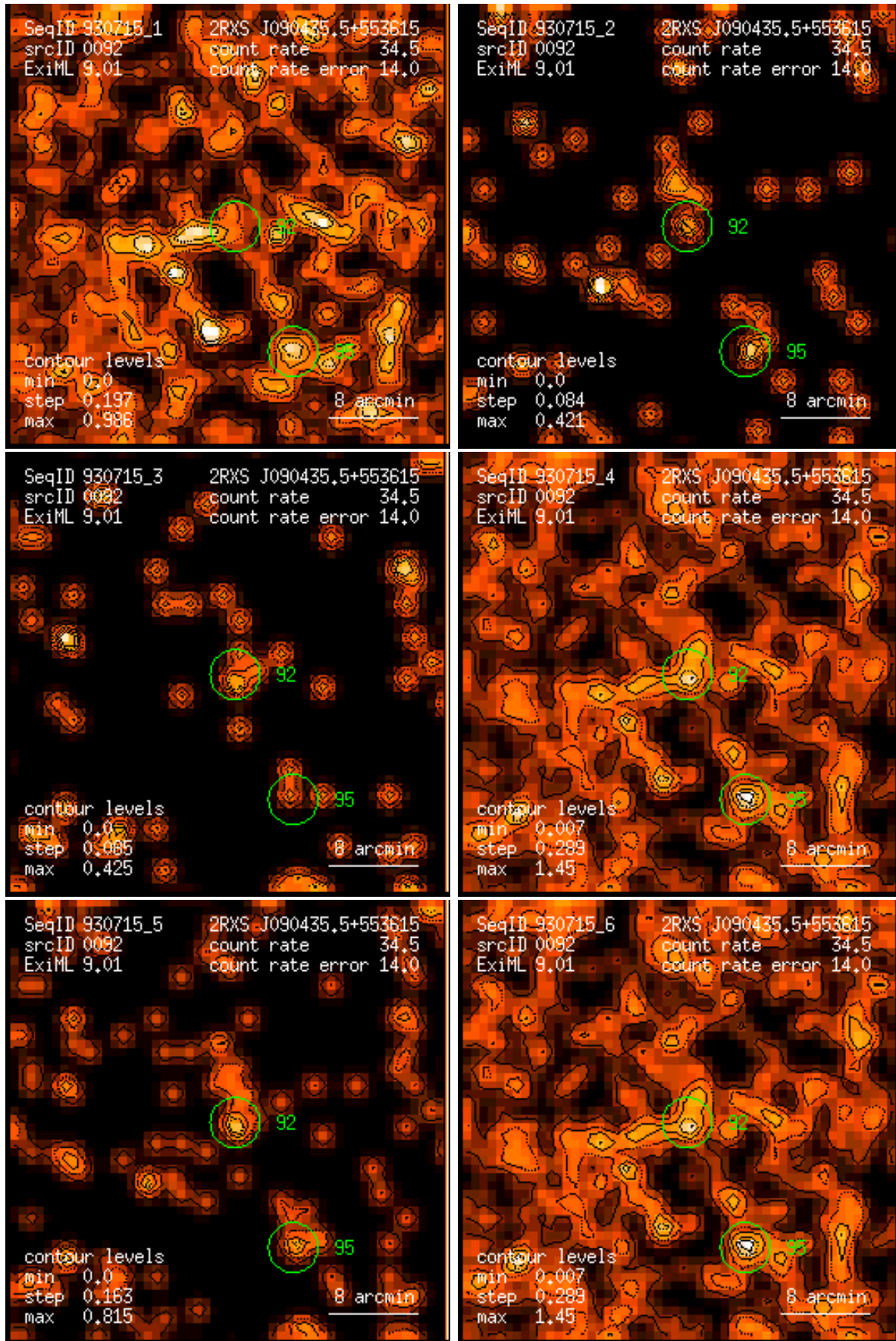
Figure 92: RASS 930715: detection 0092: band rate images, Gaussian filter: (1) PSPC channels 11 – 41, (2) 52 – 90, (3) 91 – 201, (4) 11 – 235, (5) 52 – 201, (6) 11 – 201. Broad band rates in counts/ks. Band rate contour levels in counts/ks/arcmin 2 .
