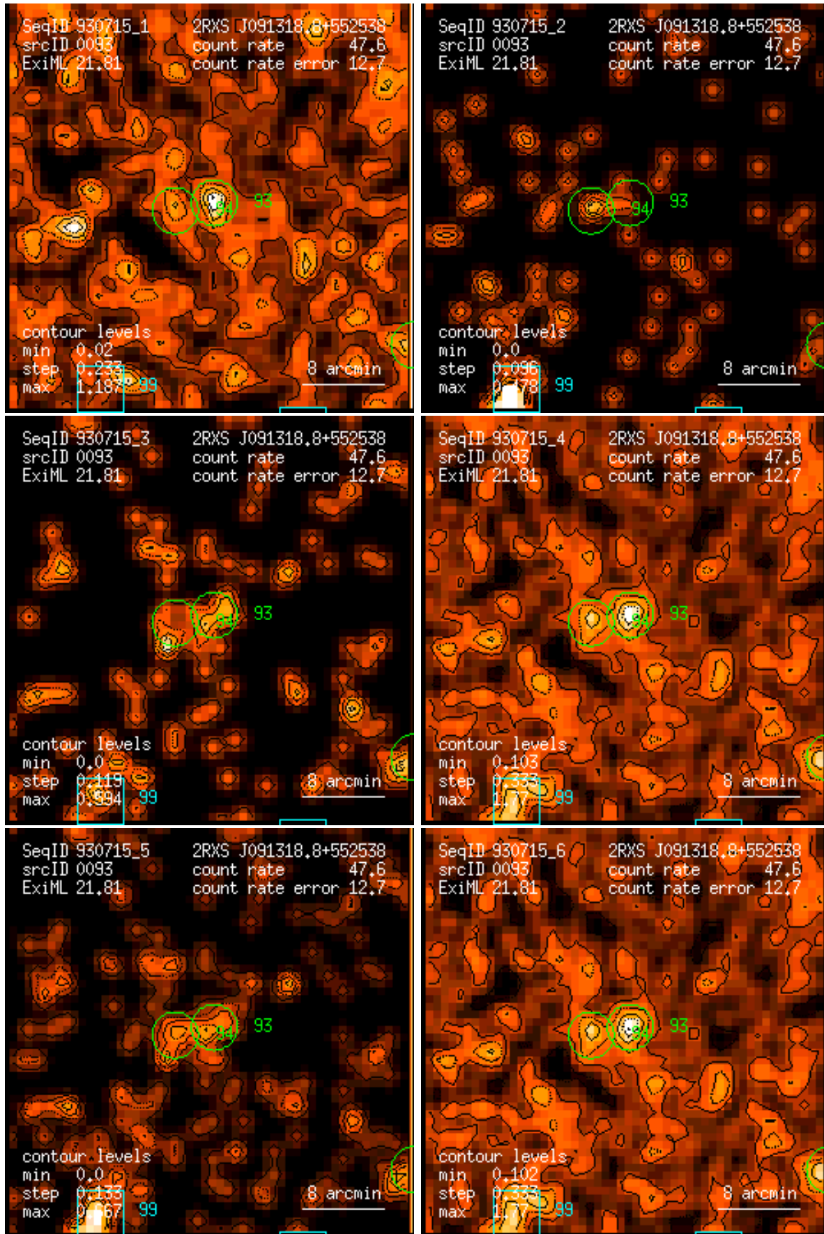
Figure 93: RASS 930715: detection 0093: band rate images, Gaussian filter: (1) PSPC channels 11 – 41, (2) 52 – 90, (3) 91 – 201, (4) 11 – 235, (5) 52 – 201, (6) 11 – 201. Broad band rates in counts/ks. Band rate contour levels in counts/ks/arcmin 2 .
