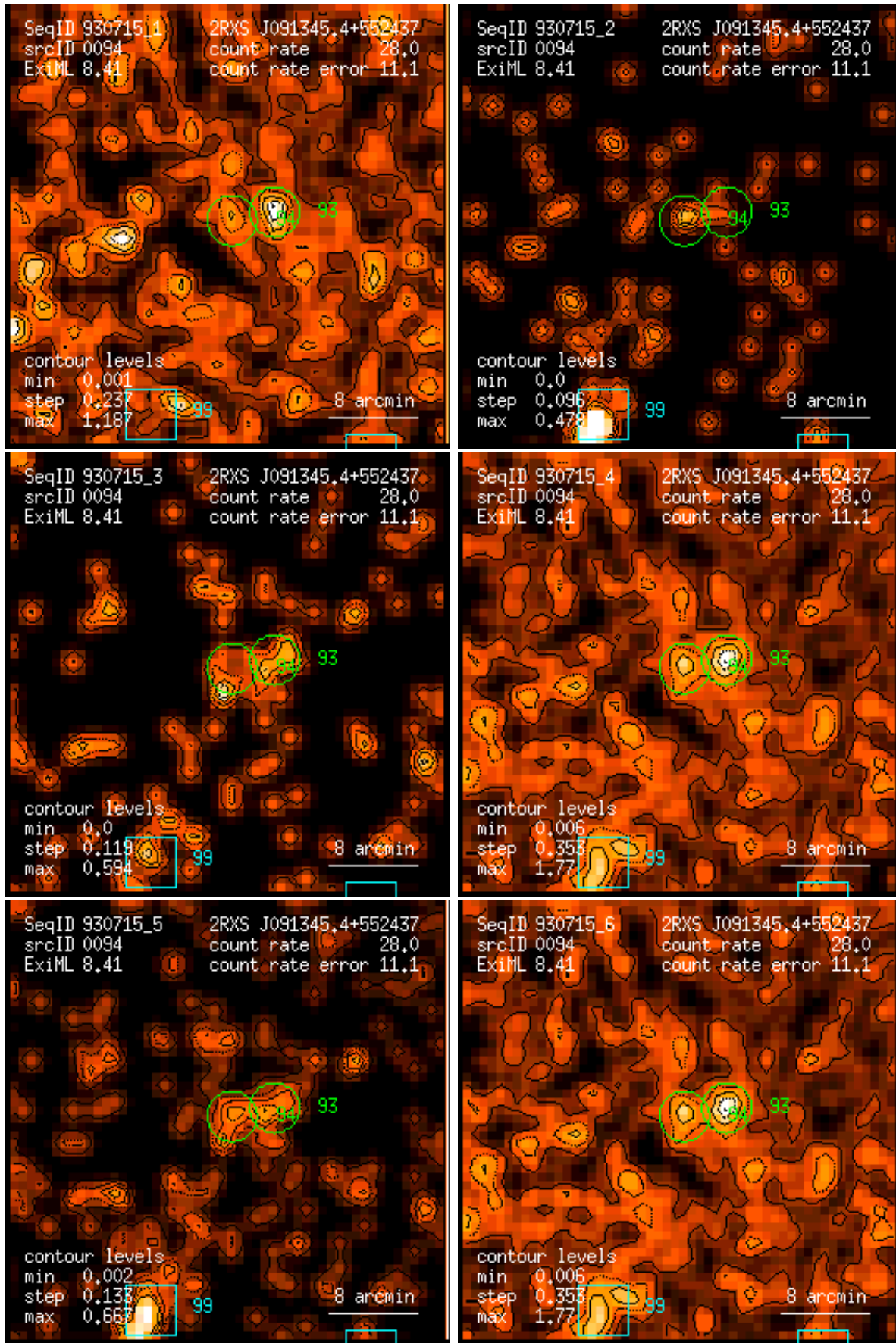
Figure 94: RASS 930715: detection 0094: band rate images, Gaussian filter: (1) PSPC channels 11 – 41, (2) 52 – 90, (3) 91 – 201, (4) 11 – 235, (5) 52 – 201, (6) 11 – 201. Broad band rates in counts/ks. Band rate contour levels in counts/ks/arcmin 2 .
