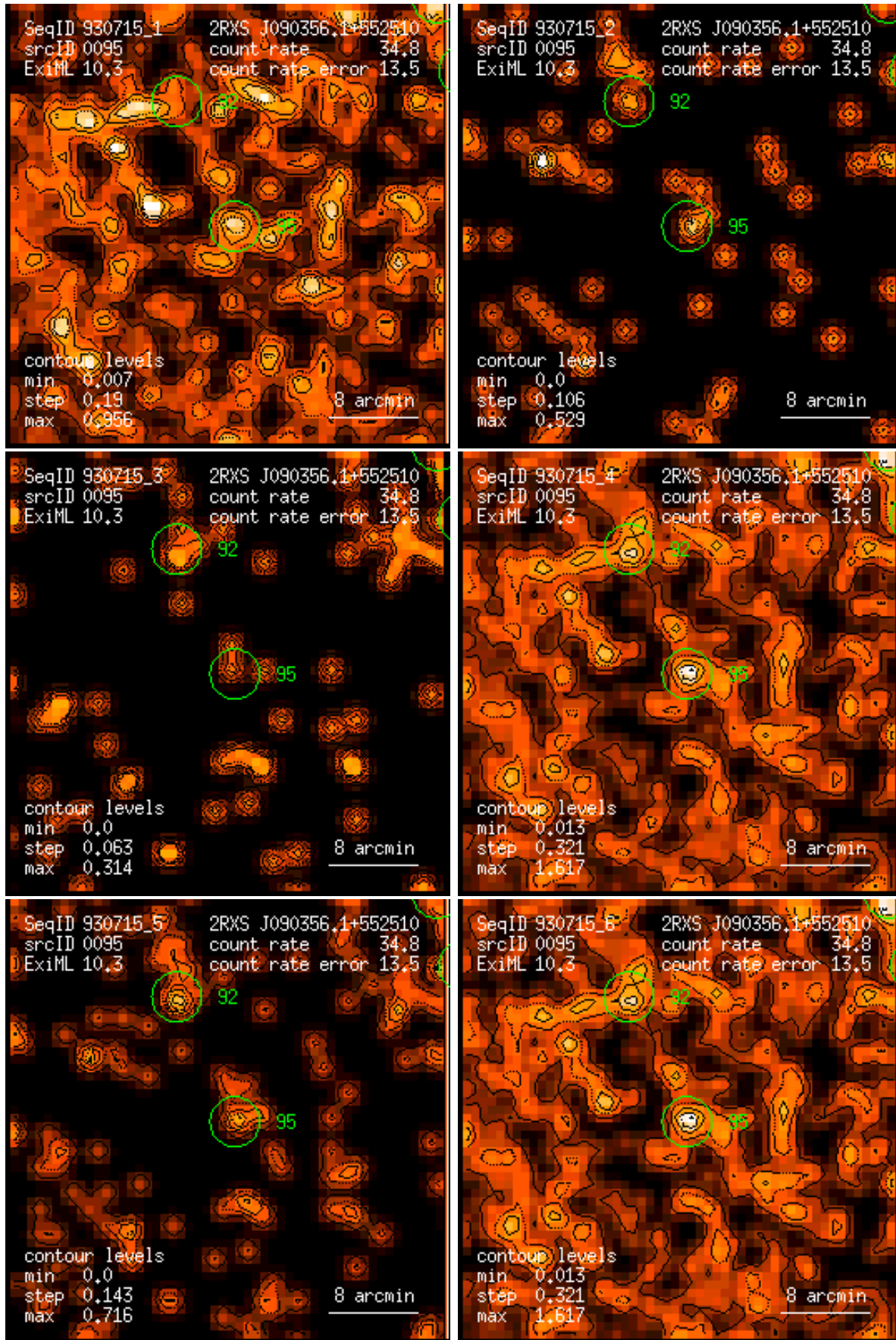
Figure 95: RASS 930715: detection 0095: band rate images, Gaussian filter: (1) PSPC channels 11 – 41, (2) 52 – 90, (3) 91 – 201, (4) 11 – 235, (5) 52 – 201, (6) 11 – 201. Broad band rates in counts/ks. Band rate contour levels in counts/ks/arcmin 2 .
