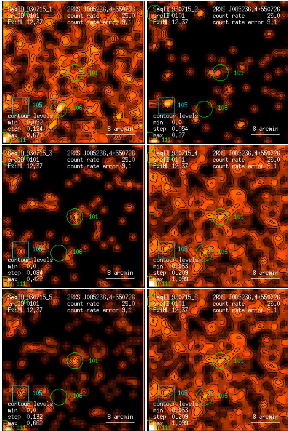
Figure 101: RASS 930715: detection 0101: band rate images, Gaussian filter: (1) PSPC channels 11 – 41, (2) 52 – 90, (3) 91 – 201, (4) 11 – 235, (5) 52 – 201, (6) 11 – 201. Broad band rates in counts/ks. Band rate contour levels in counts/ks/arcmin 2 .
