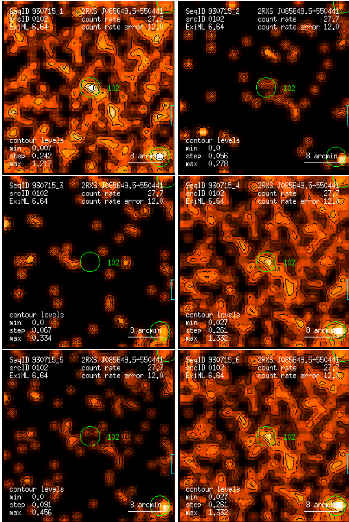
Figure 102: RASS 930715: detection 0102: band rate images, Gaussian filter: (1) PSPC channels 11 – 41, (2) 52 – 90, (3) 91 – 201, (4) 11 – 235, (5) 52 – 201, (6) 11 – 201. Broad band rates in counts/ks. Band rate contour levels in counts/ks/arcmin 2 .
