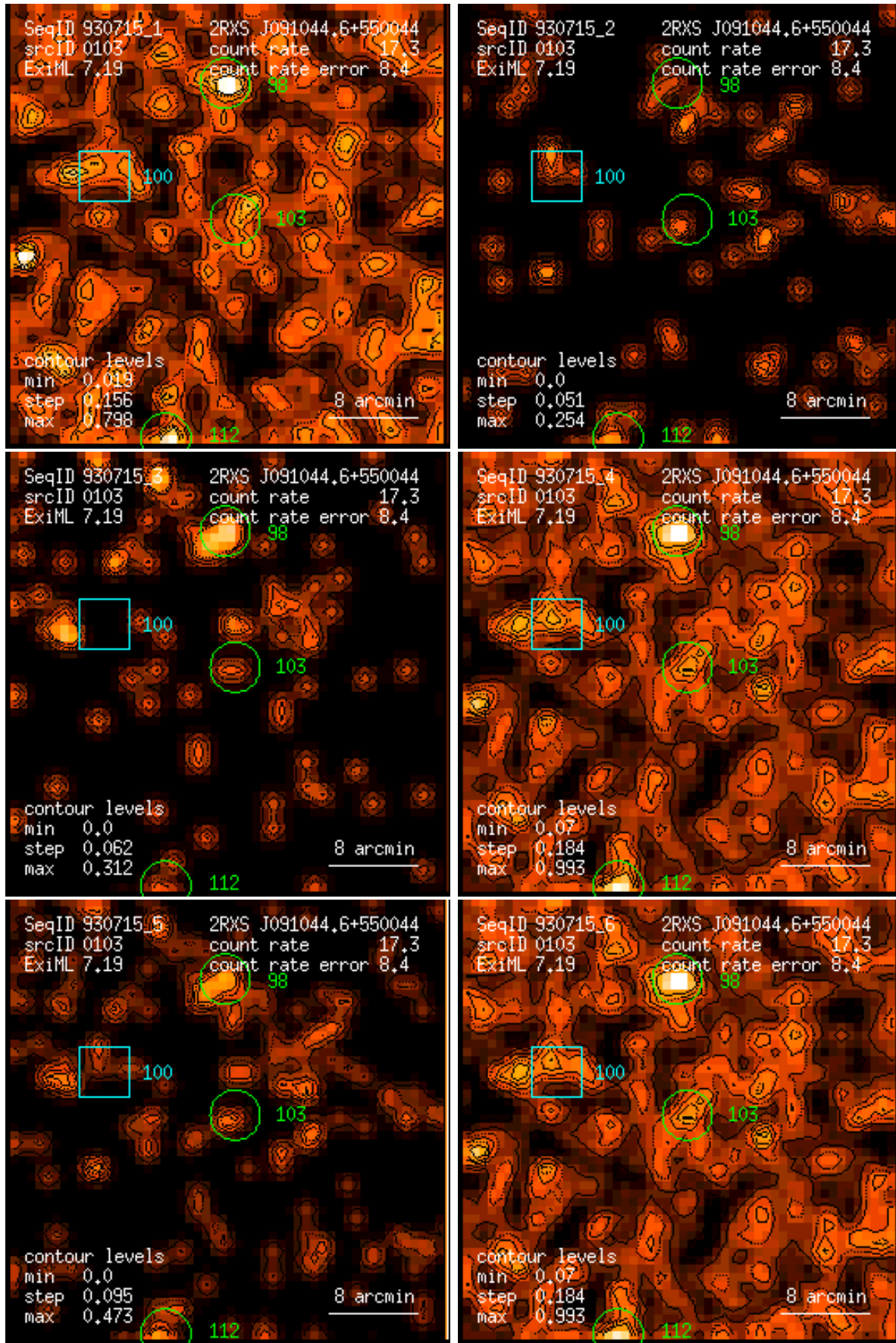
Figure 103: RASS 930715: detection 0103: band rate images, Gaussian filter: (1) PSPC channels 11 – 41, (2) 52 – 90, (3) 91 – 201, (4) 11 – 235, (5) 52 – 201, (6) 11 – 201. Broad band rates in counts/ks. Band rate contour levels in counts/ks/arcmin 2 .
