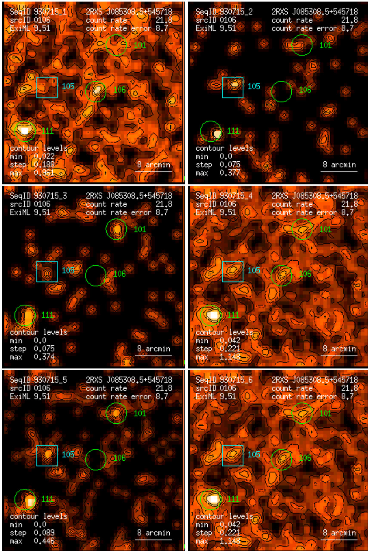
Figure 106: RASS 930715: detection 0106: band rate images, Gaussian filter: (1) PSPC channels 11 – 41, (2) 52 – 90, (3) 91 – 201, (4) 11 – 235, (5) 52 – 201, (6) 11 – 201. Broad band rates in counts/ks. Band rate contour levels in counts/ks/arcmin 2 .
