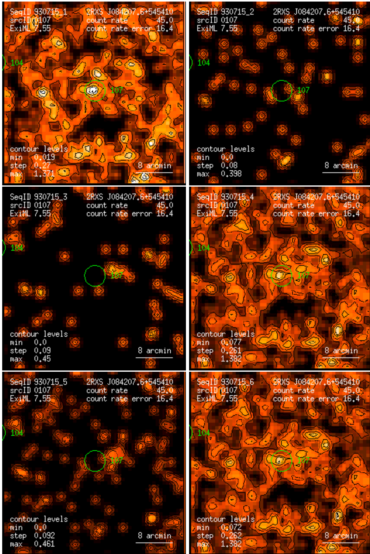
Figure 107: RASS 930715: detection 0107: band rate images, Gaussian filter: (1) PSPC channels 11 – 41, (2) 52 – 90, (3) 91 – 201, (4) 11 – 235, (5) 52 – 201, (6) 11 – 201. Broad band rates in counts/ks. Band rate contour levels in counts/ks/arcmin 2 .
