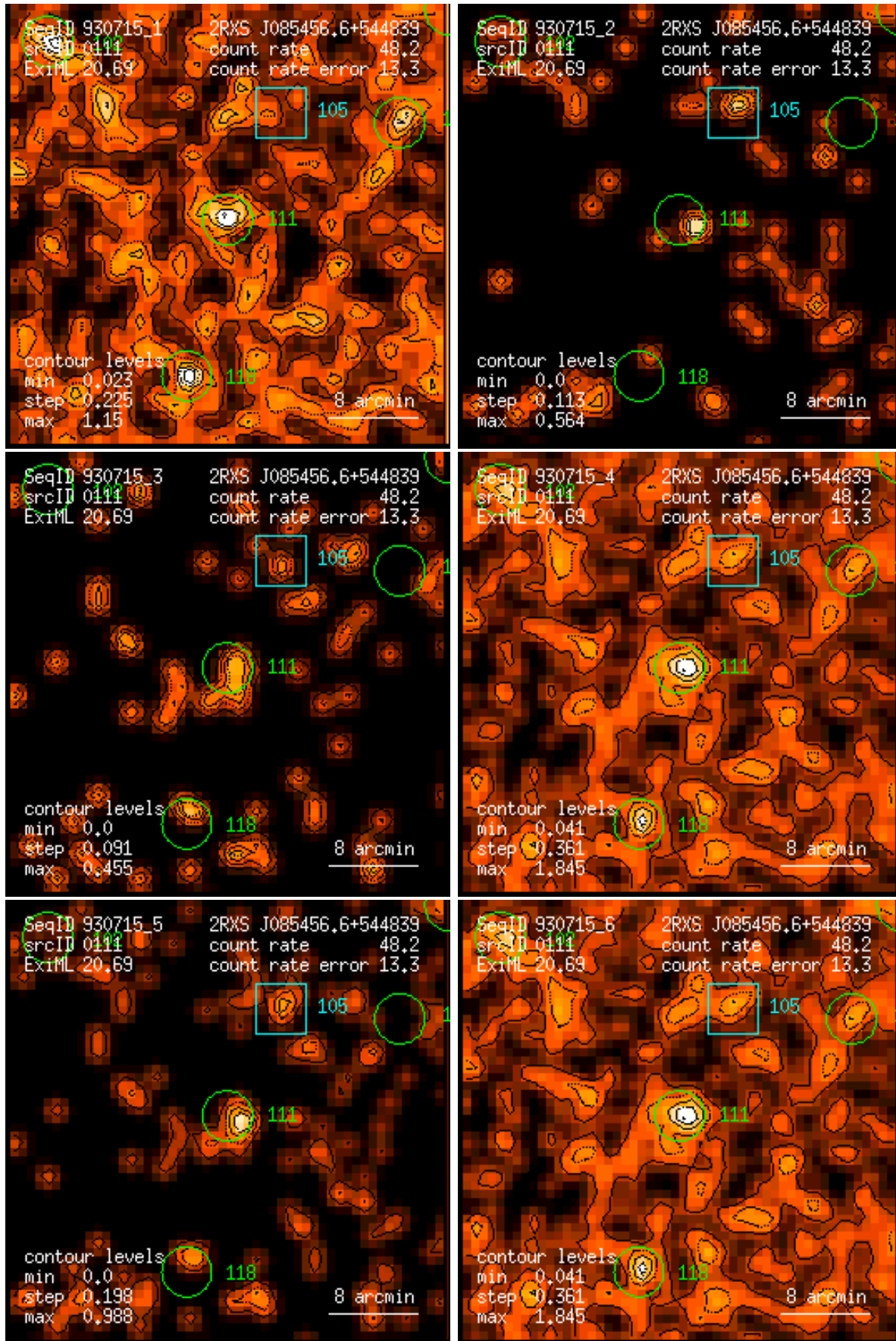
Figure 111: RASS 930715: detection 0111: band rate images, Gaussian filter: (1) PSPC channels 11 – 41, (2) 52 – 90, (3) 91 – 201, (4) 11 – 235, (5) 52 – 201, (6) 11 – 201. Broad band rates in counts/ks. Band rate contour levels in counts/ks/arcmin 2 .
