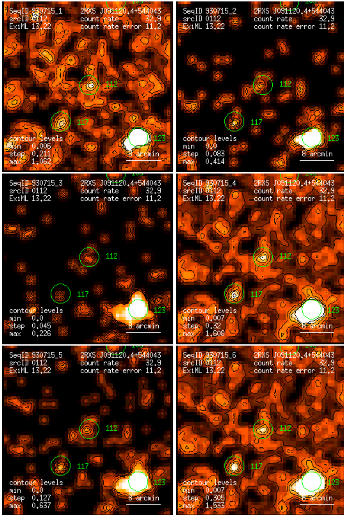
Figure 112: RASS 930715: detection 0112: band rate images, Gaussian filter: (1) PSPC channels 11 – 41, (2) 52 – 90, (3) 91 – 201, (4) 11 – 235, (5) 52 – 201, (6) 11 – 201. Broad band rates in counts/ks. Band rate contour levels in counts/ks/arcmin 2 .
