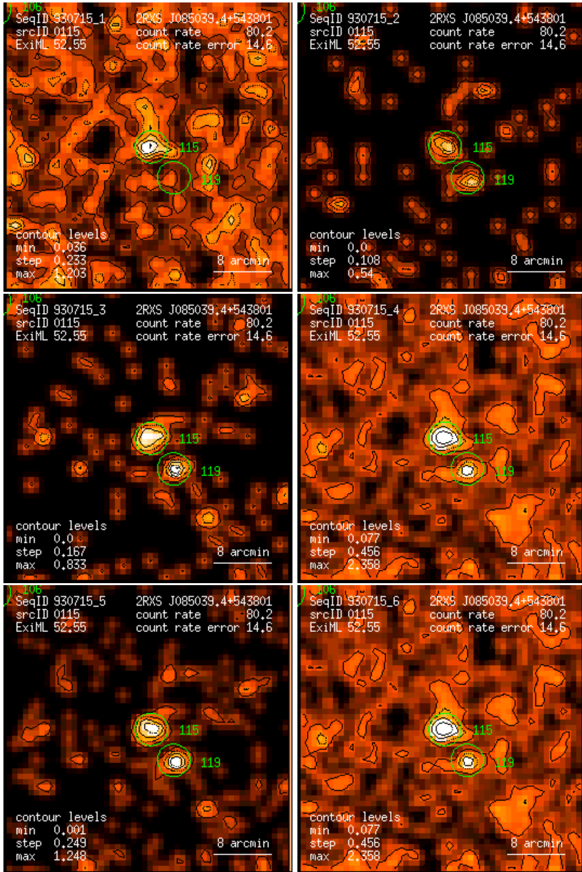
Figure 115: RASS 930715: detection 0115: band rate images, Gaussian filter: (1) PSPC channels 11 – 41, (2) 52 – 90, (3) 91 – 201, (4) 11 – 235, (5) 52 – 201, (6) 11 – 201. Broad band rates in counts/ks. Band rate contour levels in counts/ks/arcmin 2 .
