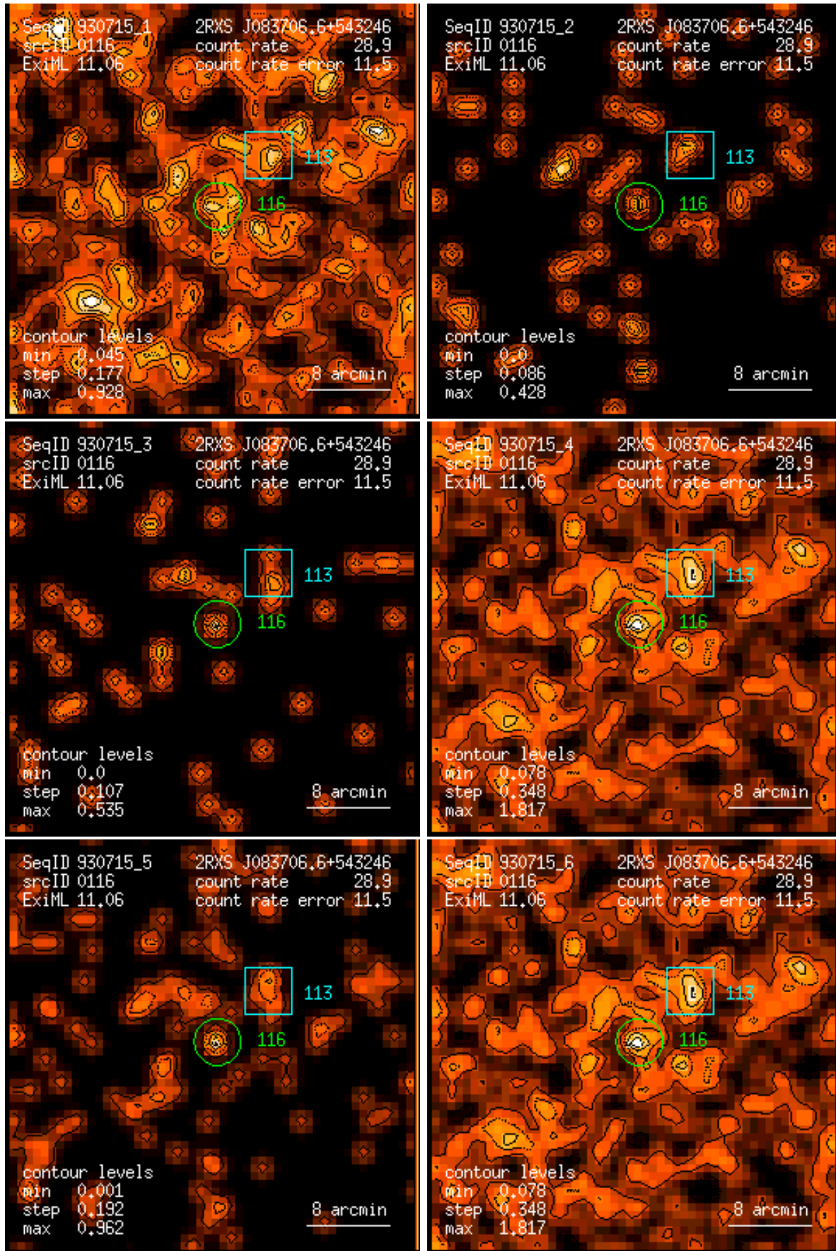
Figure 116: RASS 930715: detection 0116: band rate images, Gaussian filter: (1) PSPC channels 11 – 41, (2) 52 – 90, (3) 91 – 201, (4) 11 – 235, (5) 52 – 201, (6) 11 – 201. Broad band rates in counts/ks. Band rate contour levels in counts/ks/arcmin 2 .
