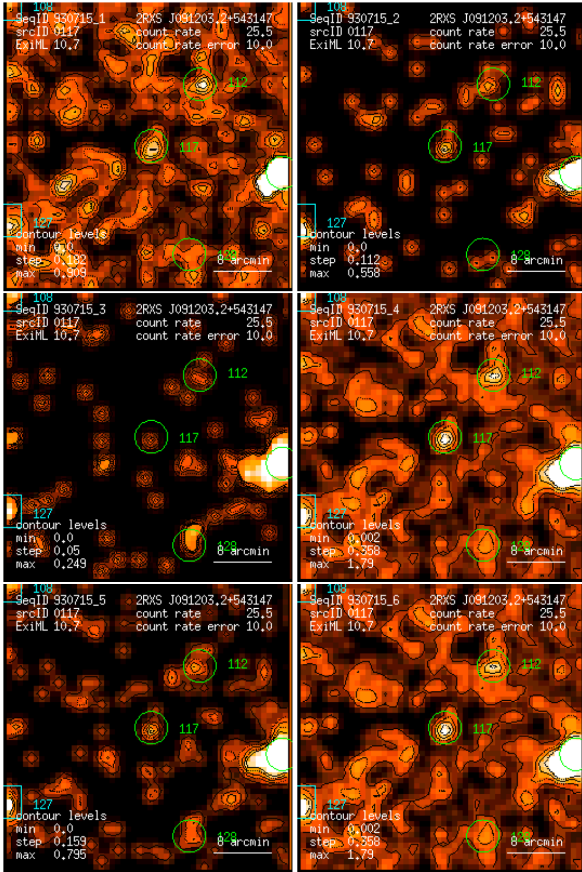
Figure 117: RASS 930715: detection 0117: band rate images, Gaussian filter: (1) PSPC channels 11 – 41, (2) 52 – 90, (3) 91 – 201, (4) 11 – 235, (5) 52 – 201, (6) 11 – 201. Broad band rates in counts/ks. Band rate contour levels in counts/ks/arcmin 2 .
