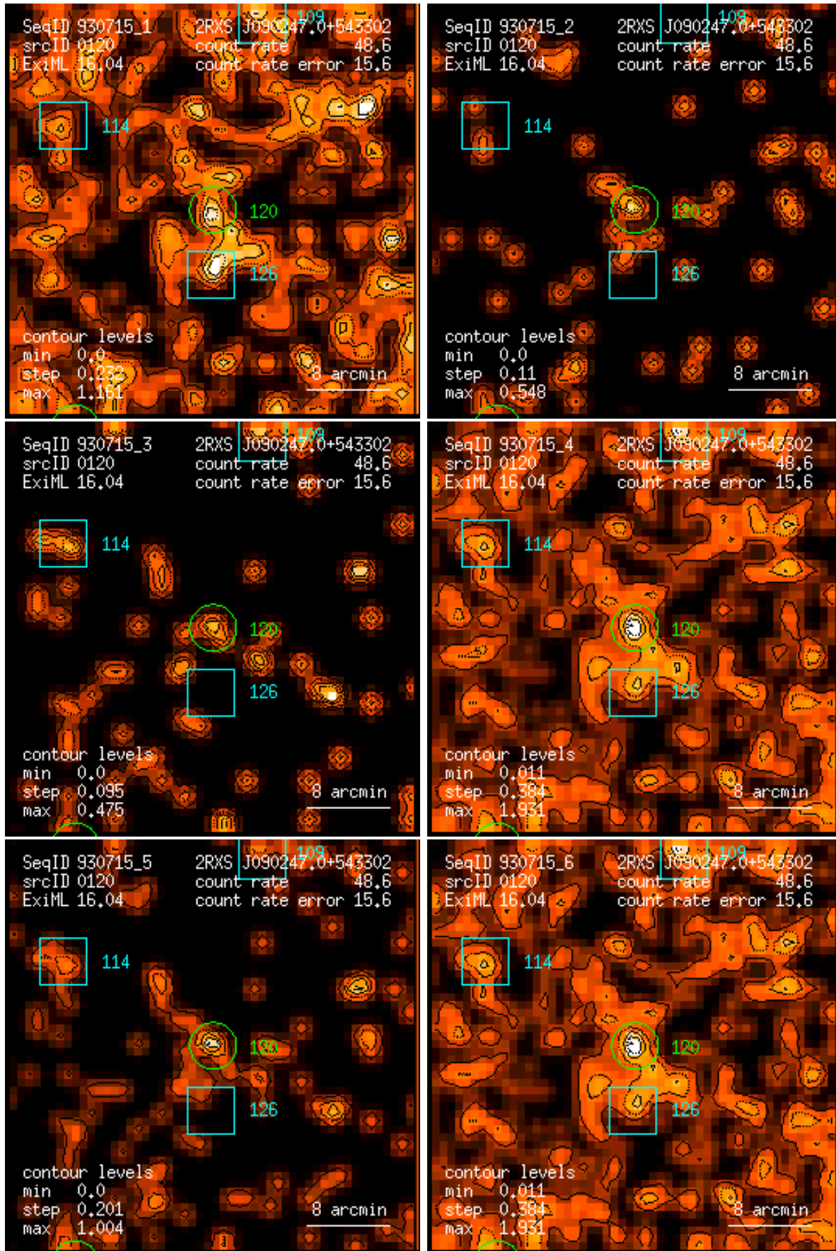
Figure 120: RASS 930715: detection 0120: band rate images, Gaussian filter: (1) PSPC channels 11 – 41, (2) 52 – 90, (3) 91 – 201, (4) 11 – 235, (5) 52 – 201, (6) 11 – 201. Broad band rates in counts/ks. Band rate contour levels in counts/ks/arcmin 2 .
