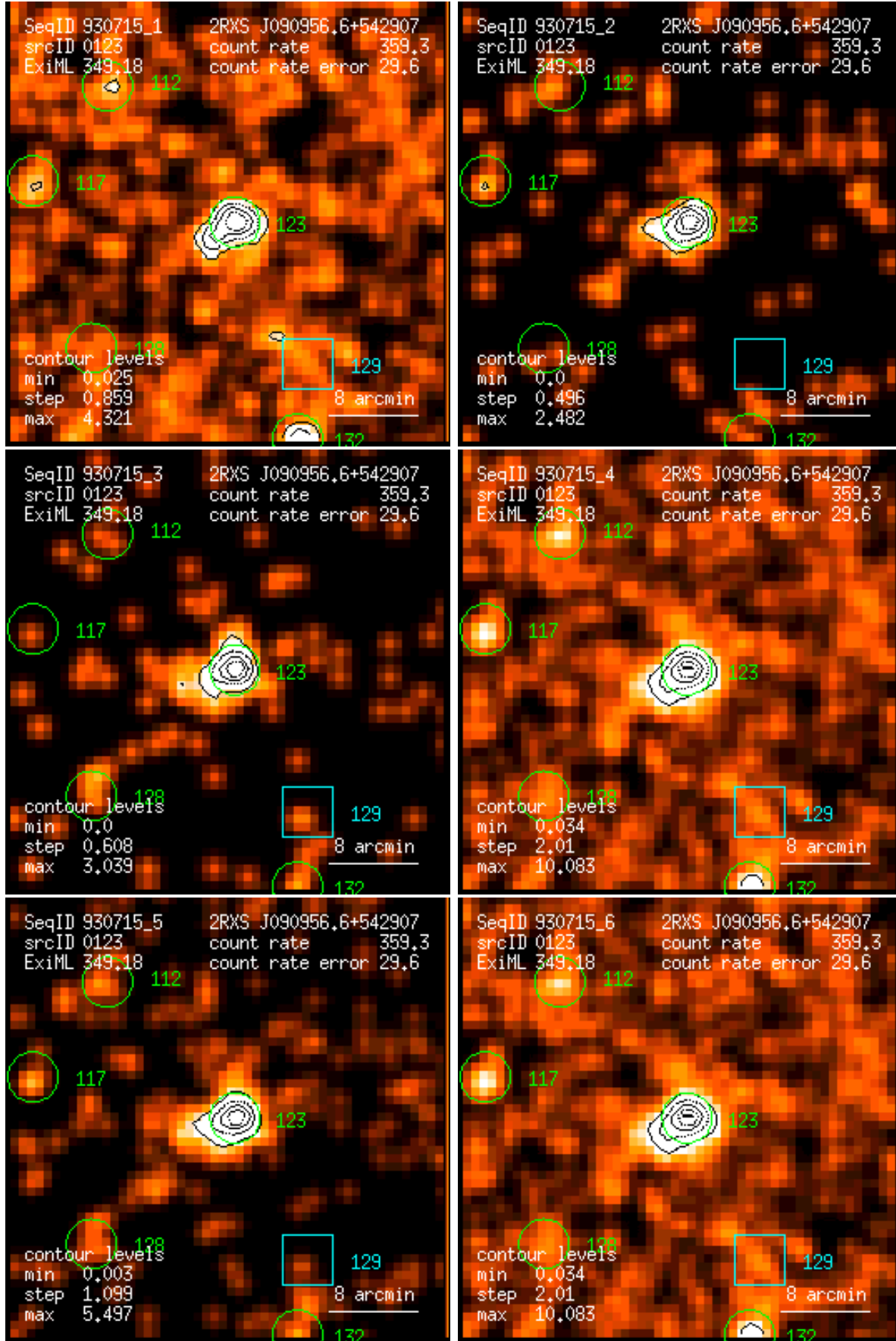
Figure 123: RASS 930715: detection 0123: band rate images, Gaussian filter: (1) PSPC channels 11 – 41, (2) 52 – 90, (3) 91 – 201, (4) 11 – 235, (5) 52 – 201, (6) 11 – 201. Broad band rates in counts/ks. Band rate contour levels in counts/ks/arcmin 2 .
