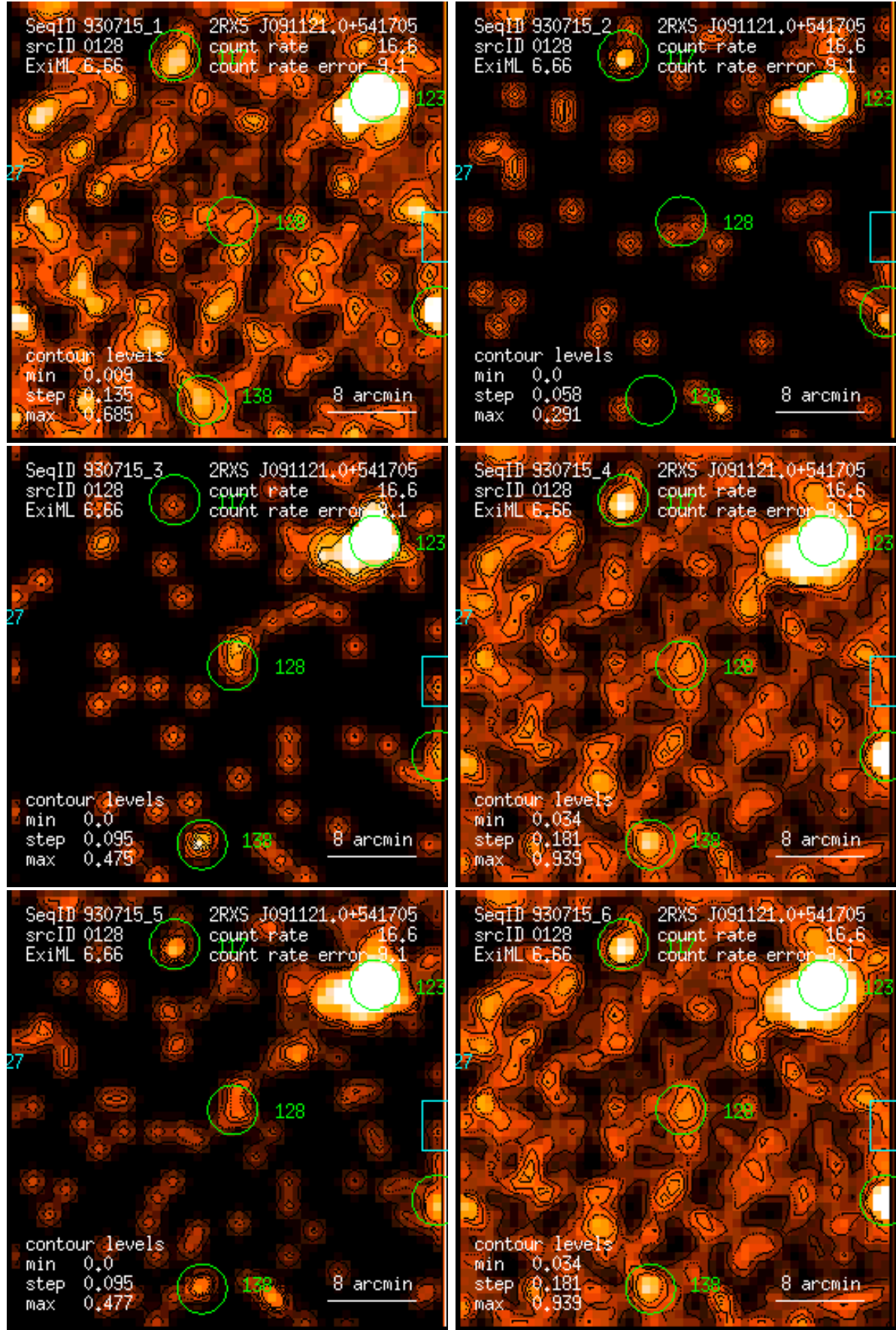
Figure 128: RASS 930715: detection 0128: band rate images, Gaussian filter: (1) PSPC channels 11 – 41, (2) 52 – 90, (3) 91 – 201, (4) 11 – 235, (5) 52 – 201, (6) 11 – 201. Broad band rates in counts/ks. Band rate contour levels in counts/ks/arcmin 2 .
