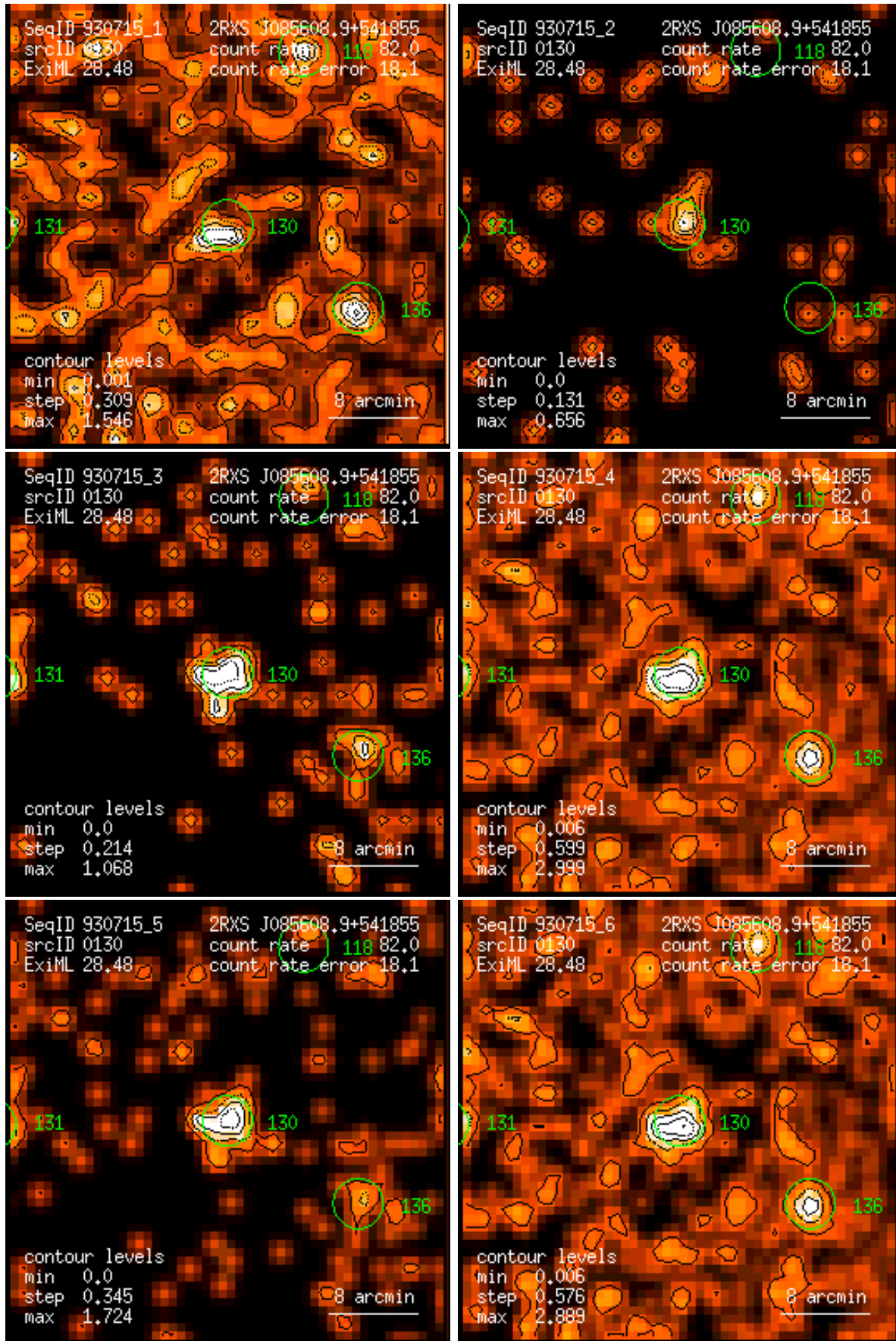
Figure 130: RASS 930715: detection 0130: band rate images, Gaussian filter: (1) PSPC channels 11 – 41, (2) 52 – 90, (3) 91 – 201, (4) 11 – 235, (5) 52 – 201, (6) 11 – 201. Broad band rates in counts/ks. Band rate contour levels in counts/ks/arcmin 2 .
