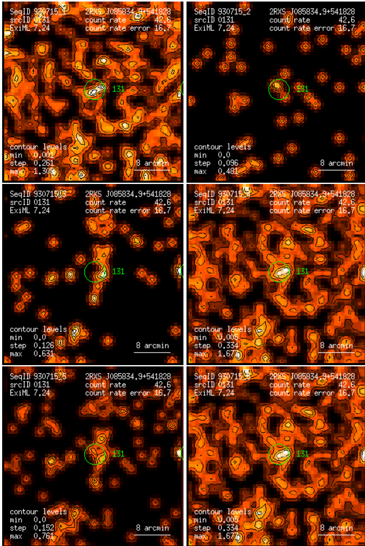
Figure 131: RASS 930715: detection 0131: band rate images, Gaussian filter: (1) PSPC channels 11 – 41, (2) 52 – 90, (3) 91 – 201, (4) 11 – 235, (5) 52 – 201, (6) 11 – 201. Broad band rates in counts/ks. Band rate contour levels in counts/ks/arcmin 2 .
