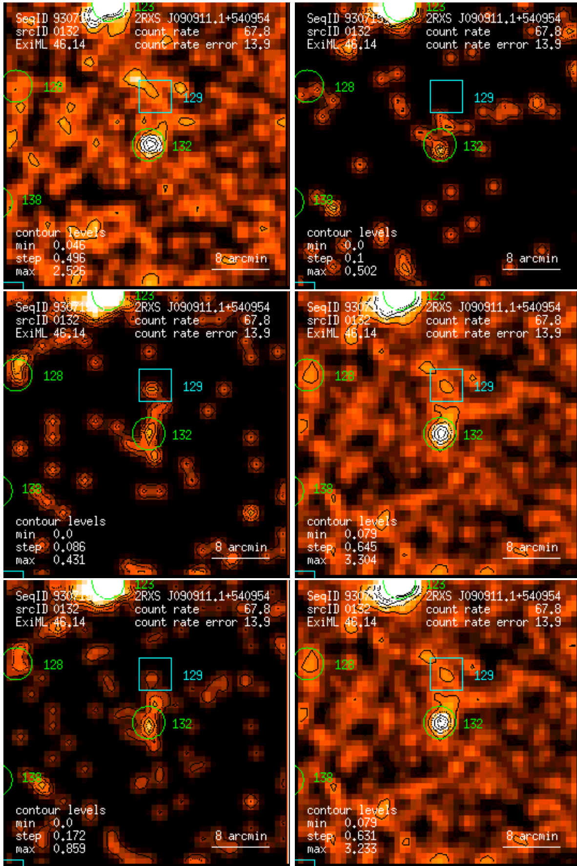
Figure 132: RASS 930715: detection 0132: band rate images, Gaussian filter: (1) PSPC channels 11 – 41, (2) 52 – 90, (3) 91 – 201, (4) 11 – 235, (5) 52 – 201, (6) 11 – 201. Broad band rates in counts/ks. Band rate contour levels in counts/ks/arcmin 2 .
