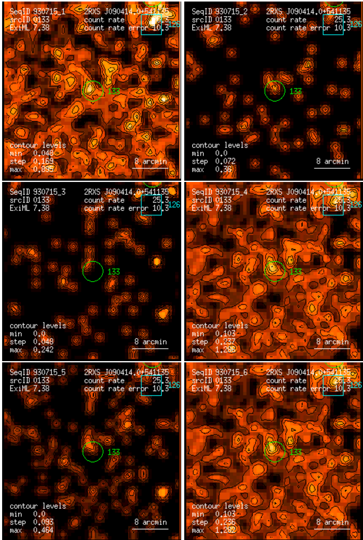
Figure 133: RASS 930715: detection 0133: band rate images, Gaussian filter: (1) PSPC channels 11 – 41, (2) 52 – 90, (3) 91 – 201, (4) 11 – 235, (5) 52 – 201, (6) 11 – 201. Broad band rates in counts/ks. Band rate contour levels in counts/ks/arcmin 2 .
