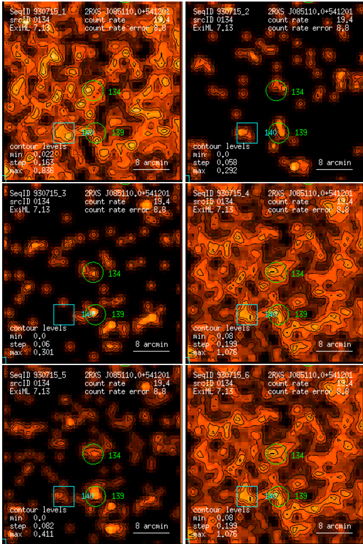
Figure 134: RASS 930715: detection 0134: band rate images, Gaussian filter: (1) PSPC channels 11 – 41, (2) 52 – 90, (3) 91 – 201, (4) 11 – 235, (5) 52 – 201, (6) 11 – 201. Broad band rates in counts/ks. Band rate contour levels in counts/ks/arcmin 2 .
