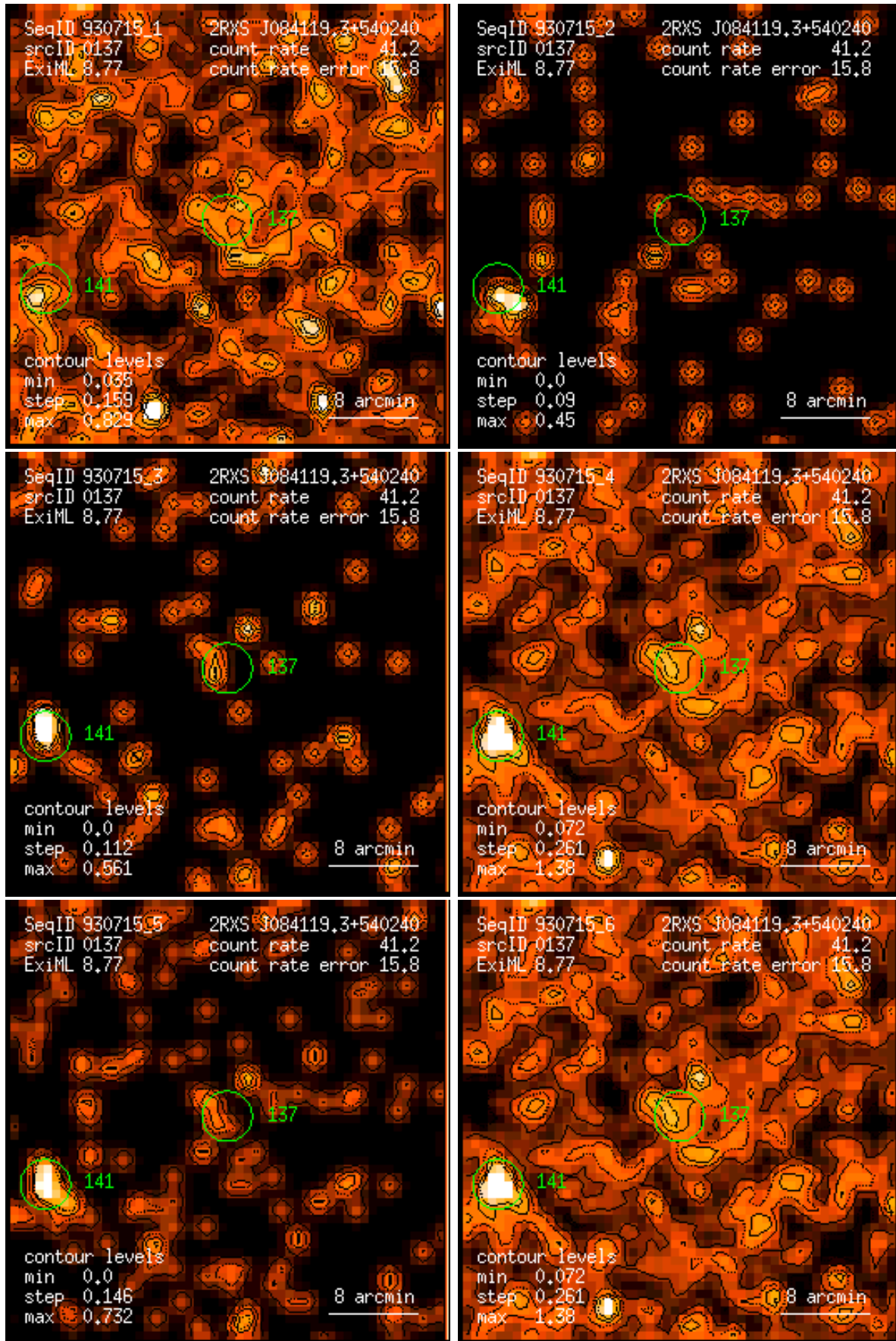
Figure 137: RASS 930715: detection 0137: band rate images, Gaussian filter: (1) PSPC channels 11 – 41, (2) 52 – 90, (3) 91 – 201, (4) 11 – 235, (5) 52 – 201, (6) 11 – 201. Broad band rates in counts/ks. Band rate contour levels in counts/ks/arcmin 2 .
