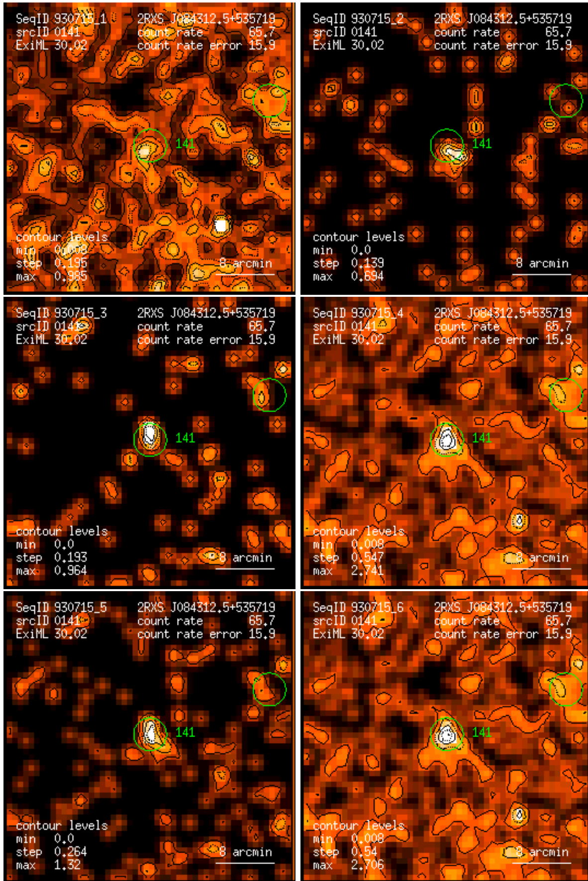
Figure 141: RASS 930715: detection 0141: band rate images, Gaussian filter: (1) PSPC channels 11 – 41, (2) 52 – 90, (3) 91 – 201, (4) 11 – 235, (5) 52 – 201, (6) 11 – 201. Broad band rates in counts/ks. Band rate contour levels in counts/ks/arcmin 2 .
