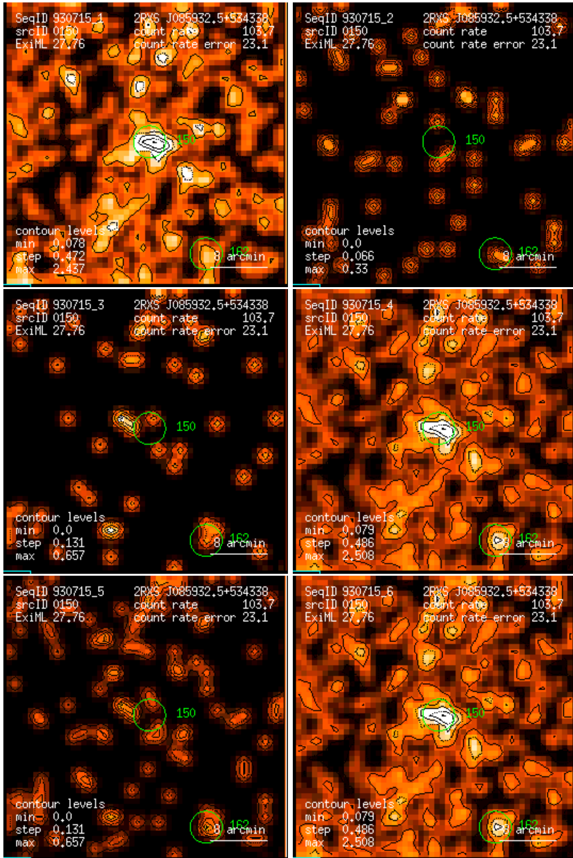
Figure 150: RASS 930715: detection 0150: band rate images, Gaussian filter: (1) PSPC channels 11 – 41, (2) 52 – 90, (3) 91 – 201, (4) 11 – 235, (5) 52 – 201, (6) 11 – 201. Broad band rates in counts/ks. Band rate contour levels in counts/ks/arcmin 2 .
