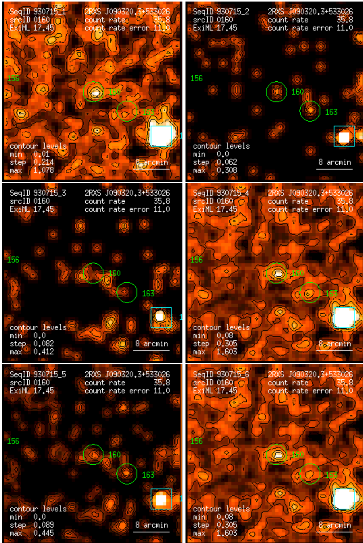
Figure 160: RASS 930715: detection 0160: band rate images, Gaussian filter: (1) PSPC channels 11 – 41, (2) 52 – 90, (3) 91 – 201, (4) 11 – 235, (5) 52 – 201, (6) 11 – 201. Broad band rates in counts/ks. Band rate contour levels in counts/ks/arcmin 2 .
