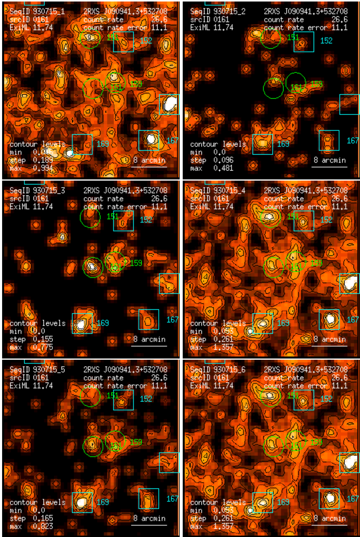
Figure 161: RASS 930715: detection 0161: band rate images, Gaussian filter: (1) PSPC channels 11 – 41, (2) 52 – 90, (3) 91 – 201, (4) 11 – 235, (5) 52 – 201, (6) 11 – 201. Broad band rates in counts/ks. Band rate contour levels in counts/ks/arcmin 2 .
