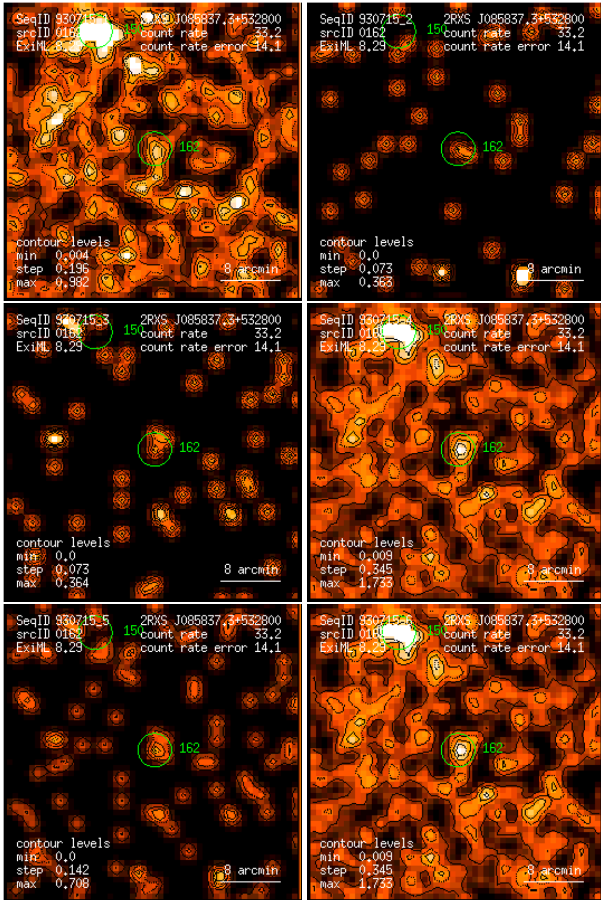
Figure 162: RASS 930715: detection 0162: band rate images, Gaussian filter: (1) PSPC channels 11 – 41, (2) 52 – 90, (3) 91 – 201, (4) 11 – 235, (5) 52 – 201, (6) 11 – 201. Broad band rates in counts/ks. Band rate contour levels in counts/ks/arcmin 2 .
