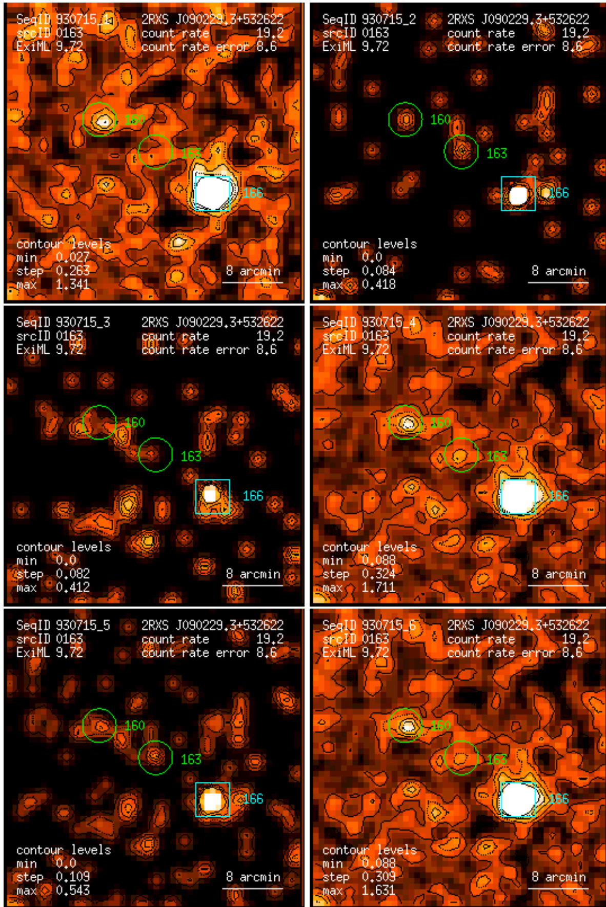
Figure 163: RASS 930715: detection 0163: band rate images, Gaussian filter: (1) PSPC channels 11 – 41, (2) 52 – 90, (3) 91 – 201, (4) 11 – 235, (5) 52 – 201, (6) 11 – 201. Broad band rates in counts/ks. Band rate contour levels in counts/ks/arcmin 2 .
