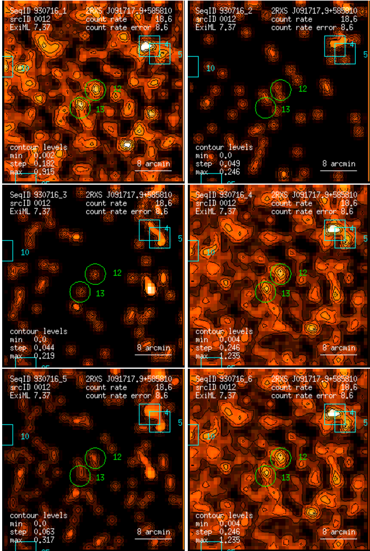
Figure 12: RASS 930716: detection 0012: band rate images, Gaussian filter: (1) PSPC channels 11 – 41, (2) 52 – 90, (3) 91 – 201, (4) 11 – 235, (5) 52 – 201, (6) 11 – 201. Broad band rates in counts/ks. Band rate contour levels in counts/ks/arcmin 2 .
