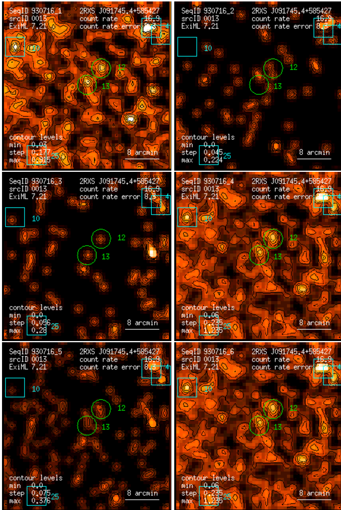
Figure 13: RASS 930716: detection 0013: band rate images, Gaussian filter: (1) PSPC channels 11 – 41, (2) 52 – 90, (3) 91 – 201, (4) 11 – 235, (5) 52 – 201, (6) 11 – 201. Broad band rates in counts/ks. Band rate contour levels in counts/ks/arcmin 2 .
